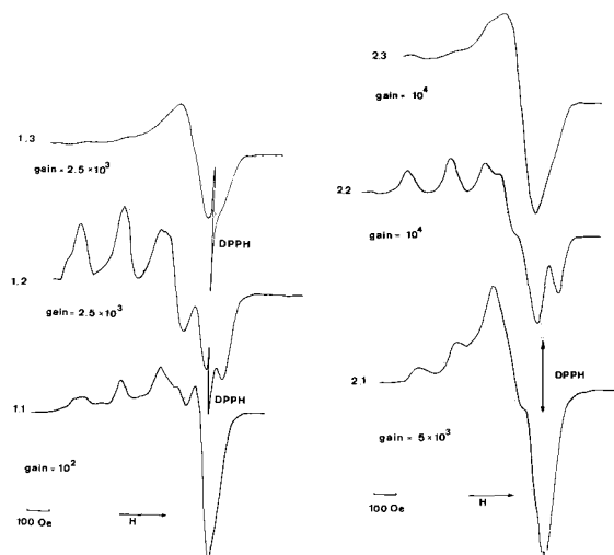
Figure 5. EPR spectra of [\text{Cu}(\text{tetren})]^{2+} at liquid nitrogen temperature. 1.1 = 10^{-3} \text{ M} \text{Cu}(\text{tetren})(\text{NO}_3)_2 in 0.1 \text{ M} \text{NaNO}_3 ; no excess ligand. 1.2 = \text{Cu}(\text{tetren})\text{H} , 10% of the CEC exchanged without pH control; c-axis parallel to magnetic field. 1.3 = as under 1.2; c-axis perpendicular to magnetic field. 2.1 = 5 \times 10^{-3} \text{ M} \text{Cu}(\text{tetren})(\text{NO}_3)_2 in 0.1 \text{ M} \text{NaNO}_3 at pH 10.30. 2.2 = \text{Cu}(\text{tetren})\text{H}_2 ; c-axis parallel to magnetic field. 2.3 = \text{Cu}(\text{tetren})\text{H}_2 ; c-axis perpendicular to magnetic field.
