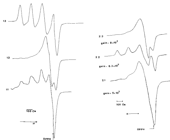
Figure 4. EPR spectra of [\text{Cu}(\text{dien})_2]^{2+} . 1.1 = 10^{-3} \text{ M} \text{Cu}(\text{dien})_2(\text{NO}_3)_2 in 0.1 \text{ M} \text{NaNO}_3 ; no excess ligand. 1.2 = \text{Cu}(\text{dien})_2\text{H} , 10% of the CEC exchanged without pH control. c-axes of the platelets parallel to the magnetic field. 1.3 = same as 1.2. c-axes of the platelets perpendicular to the magnetic field. 2.1 = 5 \times 10^{-3} \text{ M} \text{Cu}(\text{dien})_2(\text{NO}_3)_2 in 0.1 \text{ M} \text{NaNO}_3 at pH 10.30. 2.2 = \text{Cu}(\text{dien})_2\text{H}_2 with c-axis parallel to the magnetic field. 2.3 = \text{Cu}(\text{dien})_2\text{H}_2 with c-axis perpendicular to magnetic field. (Samples at liquid \text{N}_2 temperature.)
