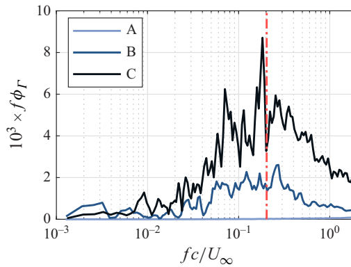
Figure 19. Premultiplied spectra of the circulation \Gamma(t) computed from the reconstructed instantaneous velocity fields for the three turbulent cases. Dash-dotted (red) line indicates normalised frequency of wing's vibration. Note that the spectral content in case A is extremely low in comparison with cases B and C.
