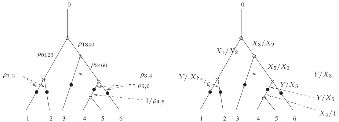
FIGURE 8. A cross-ratio chart and a simple-ratio chart for the same maximal colored tree.
