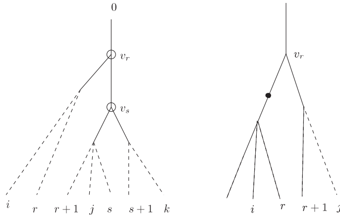
FIGURE 10. Comparing cross-ratios with simple ratios.
