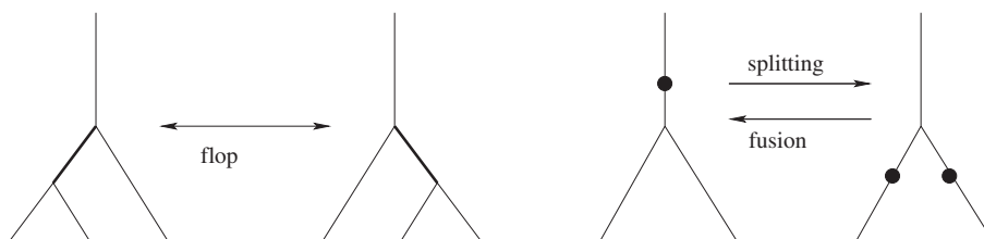
FIGURE 12. Basic moves on edges in a colored tree.
