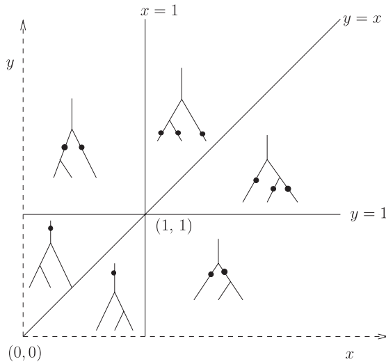
FIGURE 15. The images of the cones of W_{3,1} in the moduli space Q_3 .
