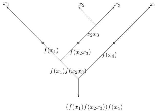
FIGURE 3. Tree for (f(x_1)f(x_2x_3))f(x_4) .
