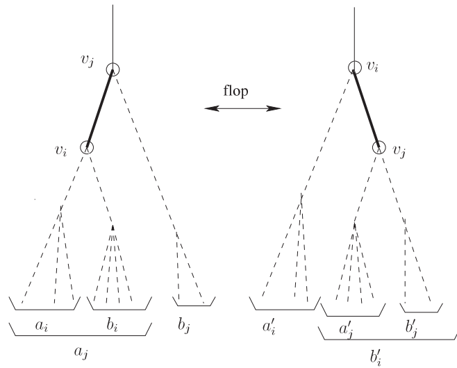
FIGURE 17. The effect of a flop on weight vectors.
