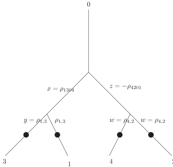
FIGURE 19. A cross-ratio chart in \overline{Q}_4(\mathbb{C}) . The relation is xy = zw , which gives a toric singularity.
