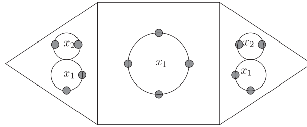
FIGURE 18. Moduli of weighted 4-marked disks.
