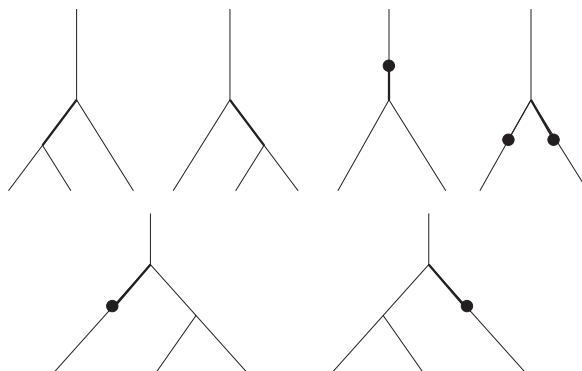
FIGURE 13. The top four types of edge have associated basic moves; the lower two types do not.
