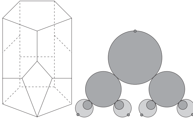
FIGURE 11. \overline{Q}_4 , sometimes called the ‘Chinese lantern’. The singular point on the boundary, which has four edges coming out of it, corresponds to the nodal quilted disk at right.
