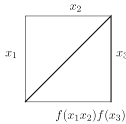
FIGURE 4. Triangulation corresponding to f(x_1x_2)f(x_3) .
