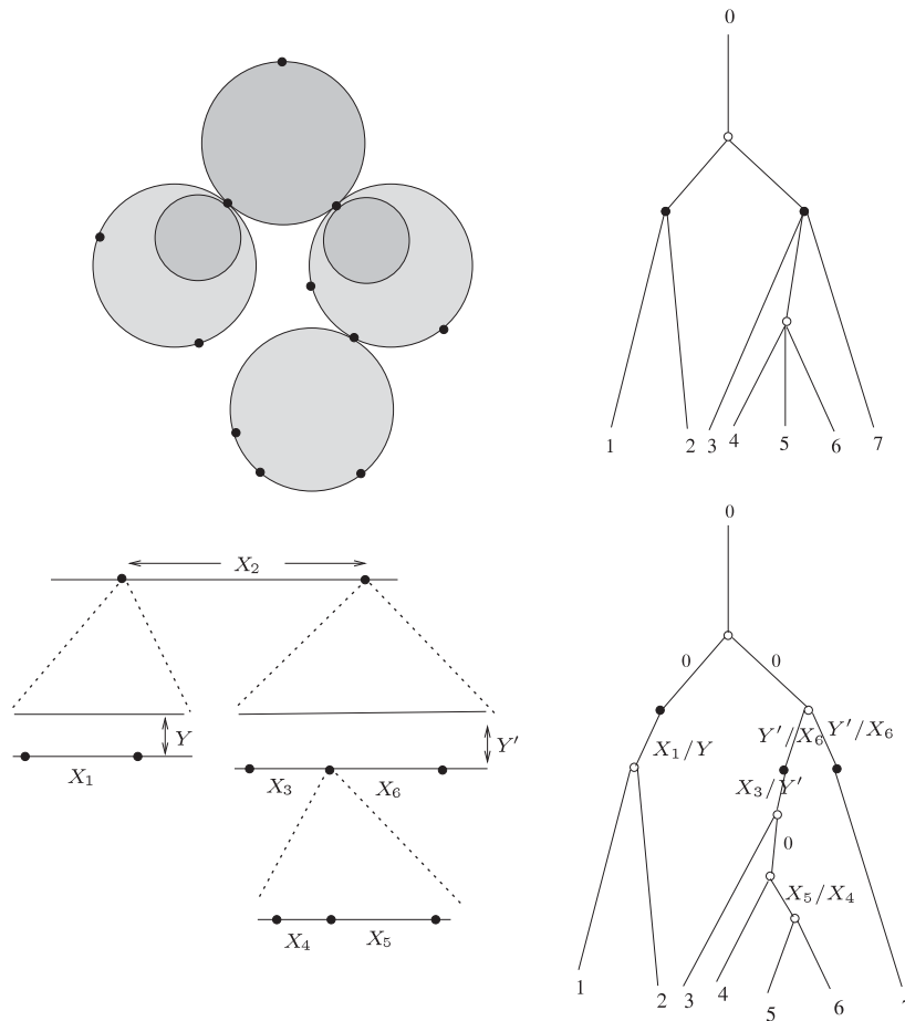
FIGURE 9. Identifying a nodal quilted disk in \overline{Q}_{7, \leq T} with a balanced labelling of T , using simple ratios.
