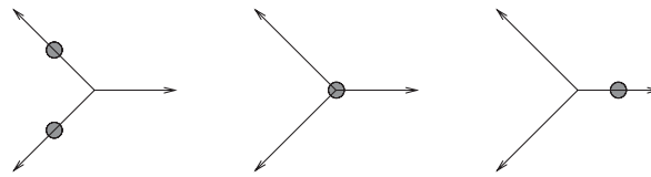
FIGURE 7. Combinatorial types for \overline{Q}_2 .
