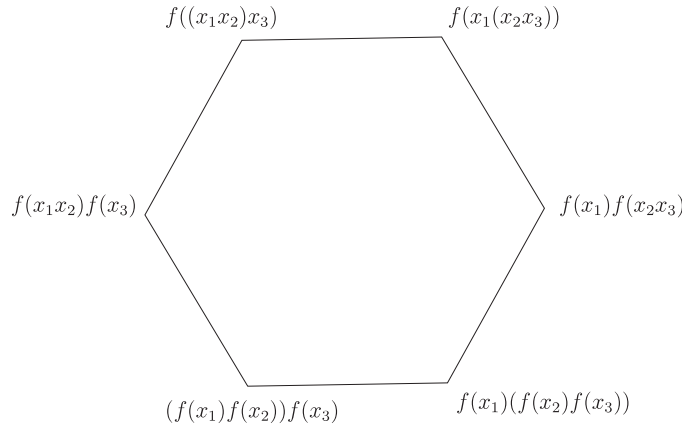
FIGURE 2. Vertices of J_3 .
