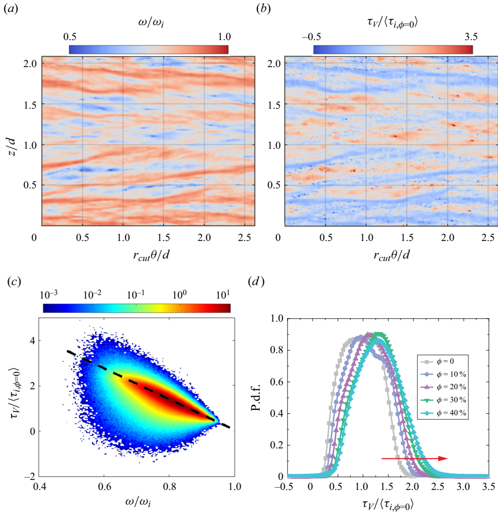
Figure 3. Contour plots of (a) the instantaneous angular velocity and (b) viscous stress on the cylinder surface with radius (r_{cut} - r_i)/d = 0.0105 for two-phase turbulence with \phi = 40\% . Here, (r_{cut} - r_i)/d = 0.0105 corresponds to y^+ = 3.45 . (c) Joint p.d.f. between the angular velocity and the viscous stress for \phi = 40\% . (d) The p.d.f.s of \tau_V for different droplet volume fractions. In (c,d), the data are sampled on the same cylinder surface as in (a,b).
