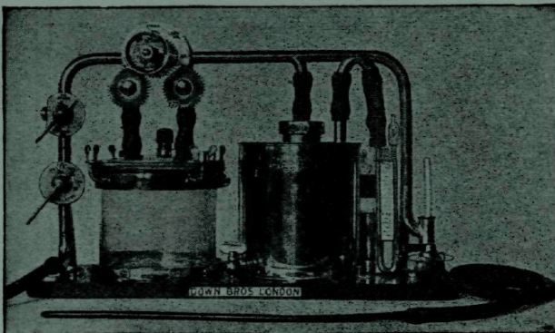
Etherization Apparatus.
