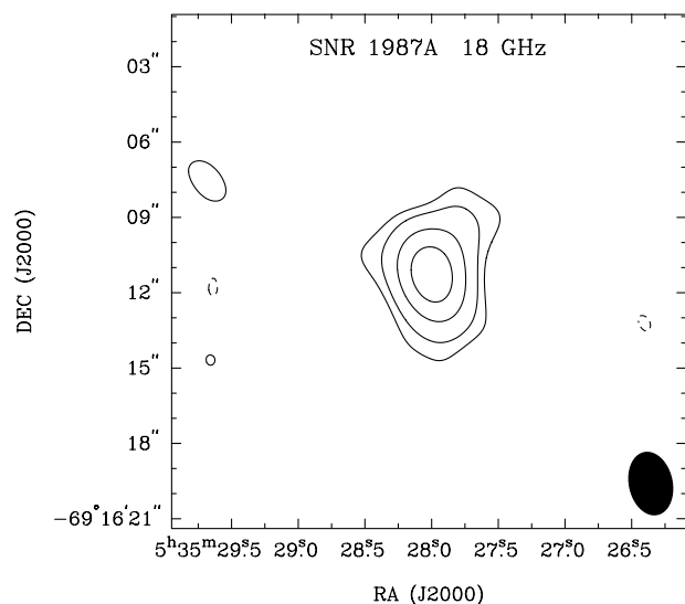
Figure 3 Image of the remnant of SN 1987A derived from a 10-h synthesis at the ATCA. Data from two frequencies (17 and 19 GHz) have been combined. The synthesised beam ( 2''.8 \times 1''.8 ) is shown at the lower right. The contour levels are -1, 1, 2, 5, and 10 \text{ mJy beam}^{-1} . Courtesy R. Manchester.
