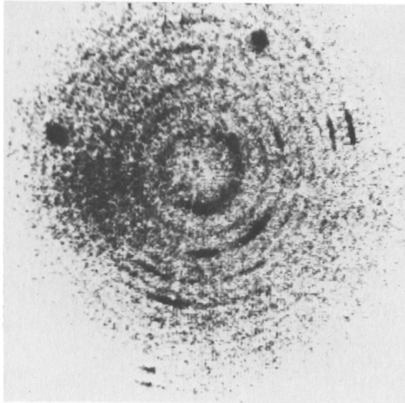
Figure 1. Interferogram of M33 in NII light. 2^h exposure time. Southern part of the galaxy (inverse image).
