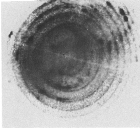
Figure 2. Interferogram of NGC 2903 in H\alpha light (inverse image): 1 h 30 exposure time.
