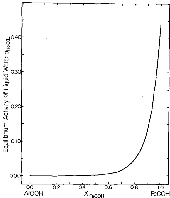
Figure 1. Plot of the calculated activity of liquid water in equilibrium with goethite-diaspore and \text{Fe}_2\text{O}_3\text{-Al}_2\text{O}_3 ideal solid solutions as a function of the mole fraction of FeOOH in the goethite. The actual range of X_{\text{FeOOH}} over which this curve is likely to be valid for natural samples is about 0.68 to 1.00 (see text).
