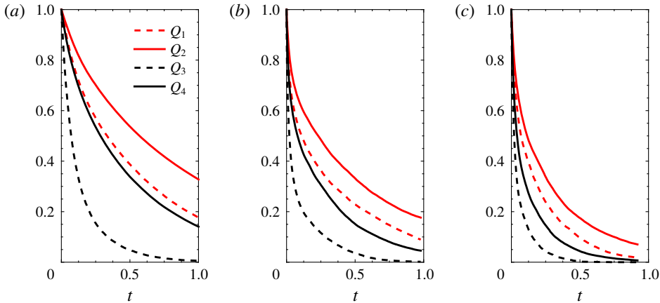
FIGURE 20. (Colour online) Percentage of fluid particles that stay in each quadrant following particles initialized uniformly in (a) isotropic turbulence and (b) single-fluid and (c) multi-fluid turbulence at post-shock position of k_0x = 0.44 .
