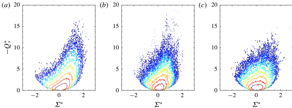
FIGURE 18. (Colour online) Iso-contour lines of joint PDF of (-Q_s^*, \Sigma^*) for (a) isotropic box turbulence and (b) single-fluid and (c) multi-fluid turbulence at post-shock position of k_0x \approx 0.44 .
