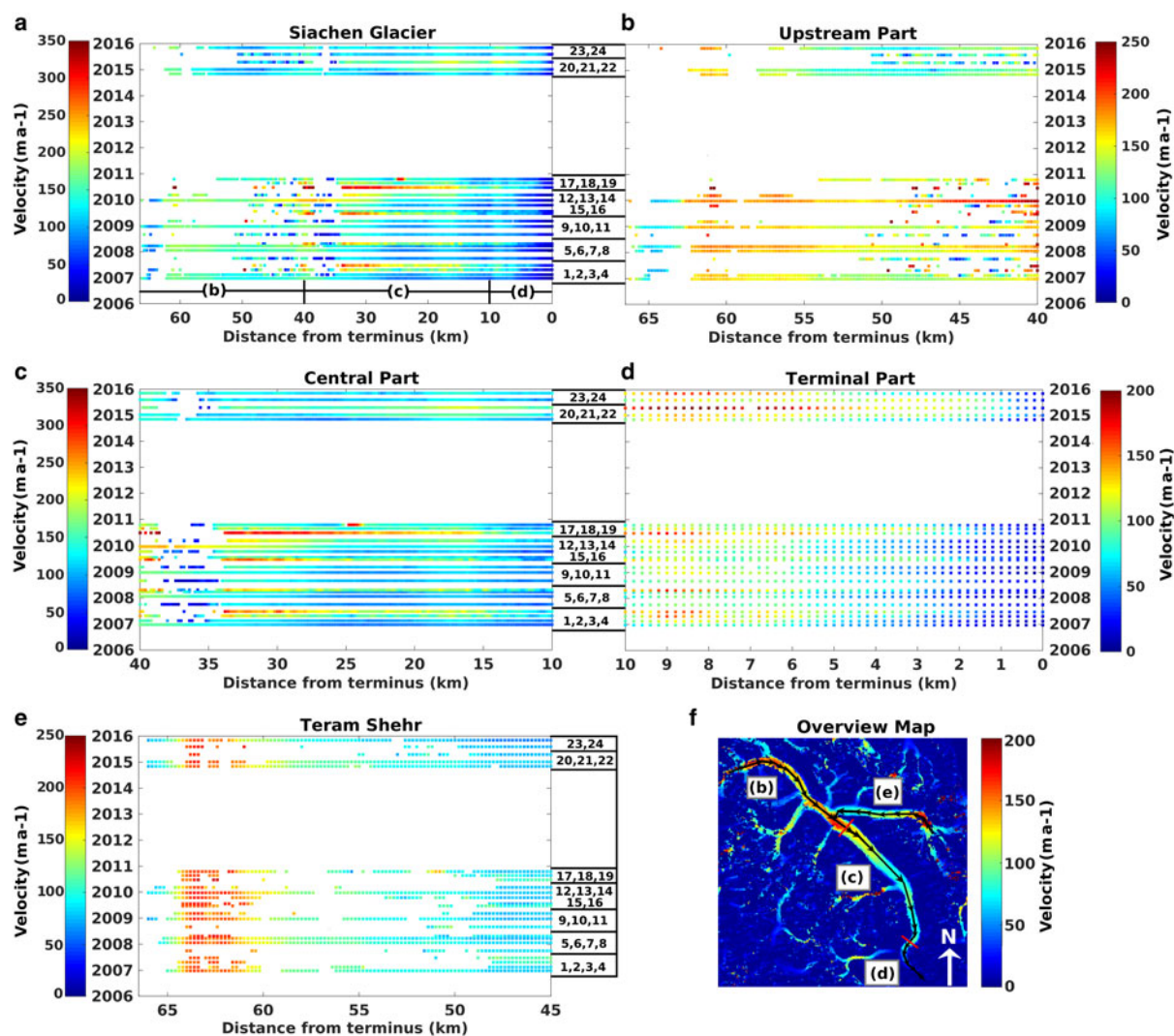
Fig. 3. (a) Spatial and temporal surface velocity changes extracted along the entire length of the centerline of the Siachen Glacier. Expanded view of individual centerline segments of Siachen Glacier; (b) upstream portion (66–40 km), (c) central portion (40–10 km), (d) terminal portion (10–0 km) and (e) the Teram Shehr tributary (red lines indicate the boundary of each segmented centerline portion). The color scale in (a, b, c, d, e, f) indicates the scale for the velocity of the glacier, its various parts and of the overview map. The numbers between the color scales and velocity figures indicate the time in years, and they are labeled at the start of the year, i.e. January. The numbers between the vertical axes of the velocity figures, i.e. between (a) and (b), (c) and (d) and on the right side of figure (e), indicate the corresponding analyzed pair results of master-slave images. The details of the respective pair dates are given in Table 1 and the corresponding velocity field of each pair is given in Figure S2. (f) Surface velocity snapshot of Siachen Glacier derived from 6 December 2006 and 21 January 2007 data. The black line shows the profile line along which the velocity was calculated and arrows indicate the flow direction of the glacier.
