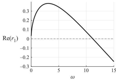
Figure 6. Spatial growth per unit length (real part of r_1 ) as a function of driving frequency \omega at \alpha = 5 . For dimensional units, r_1/L^* will yield units of 1/length; \omega/t^* will yield units 1/time.
