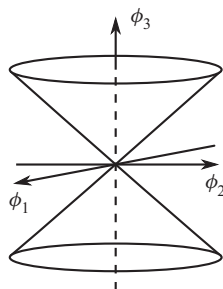
Figure 1. Elliptic cone.
