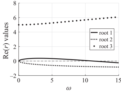
Figure 4. Spatial growth per unit length: real part (Re) of roots r_1 , r_2 and r_3 (as per (4.8)) for \alpha = 5 and as a function of driving frequency \omega . For dimensional units, R(r)/L^* will yield units of 1/length; \omega/t^* will yield units 1/time.
