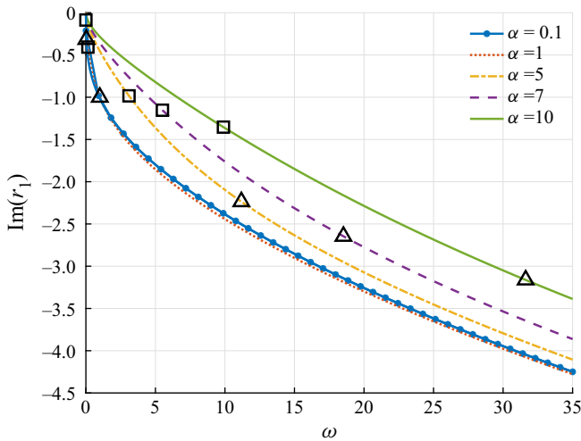
Figure 16. Wavenumber ( \text{Im}(r_1) ) as a function of driving frequency \omega at various values of \alpha . Squares mark conditions for maximum spatial growth. Triangles mark conditions for neutral stability. For each line, values left (right) of the corresponding triangle correspond to regions of spatial growth (decay).
