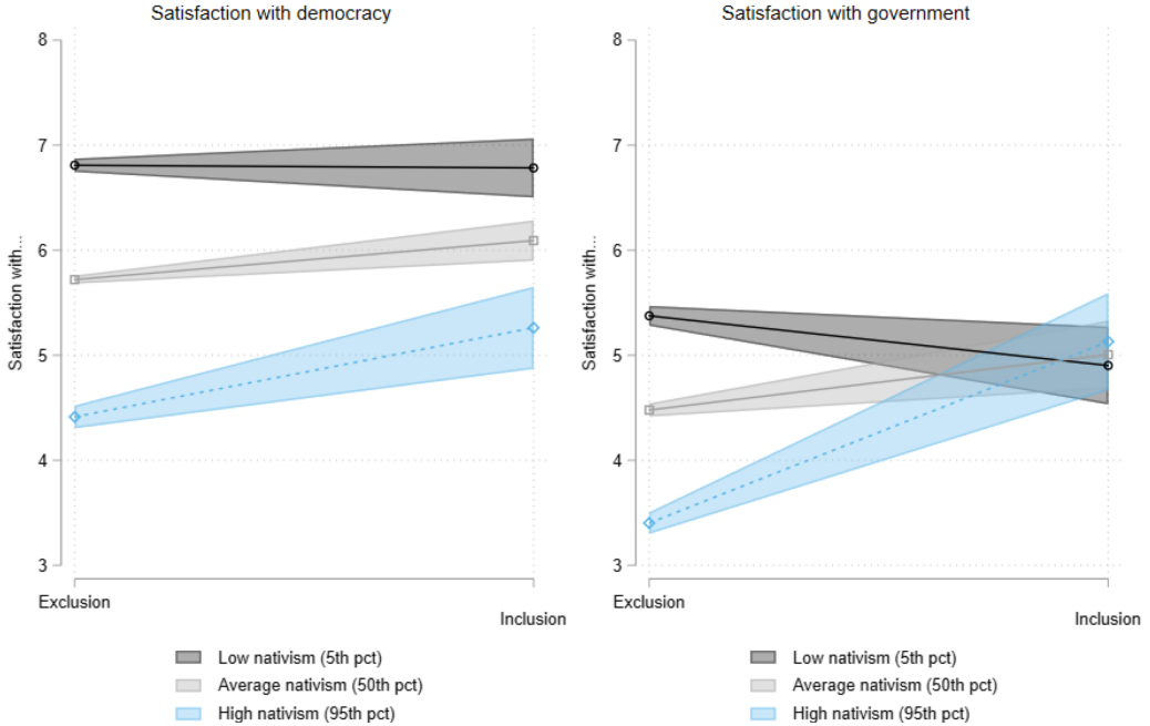
Figure 4. The effect of inclusion on satisfaction with democracy and government (ESS). Source: European Social Survey. Note: Based on models hyb3 in Table 2.
