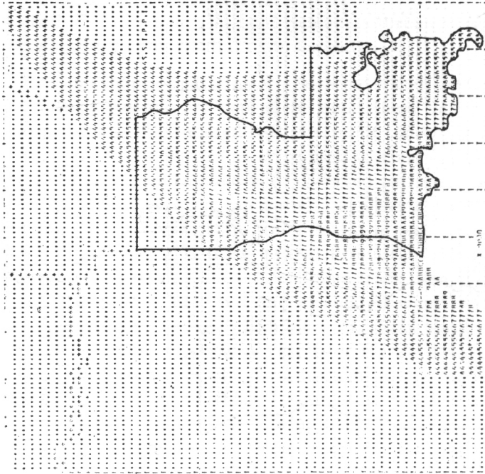
Exhibit 13. (continued) Observed and calculated geographical pattern of highest wind associated with passage of Hurricane Audrey across the Gulf Coastline in 1957.
