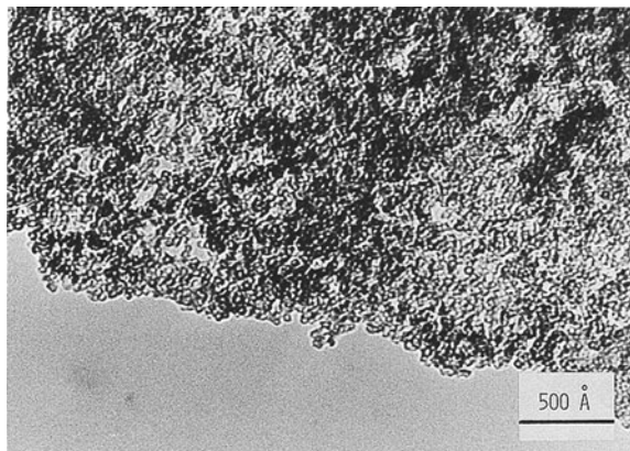
Figure 4. Transmission electron micrograph of allophane (Ki-P) heated at 500°C.
