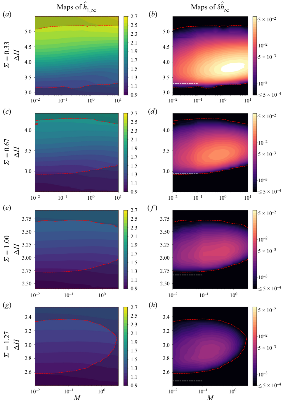
Figure 7. Asymptotic thicknesses \hat{h}_{1,\infty} (lower film, a,c,e,g ) and \delta\hat{h}_{\infty} (upper film, b,d,f,h ), shown as colour contour maps in the (M, \Delta H) parameter space. Each row corresponds to a different surface tension ratio \Sigma . The red dashed lines enclose the ‘existence islands’ of a double coating, namely the areas in the parameter space where \delta\hat{h}_{\infty} \geq 5 \times 10^{-4} . The values of \hat{h}_{1,\infty} obtained outside these islands are shaded.
