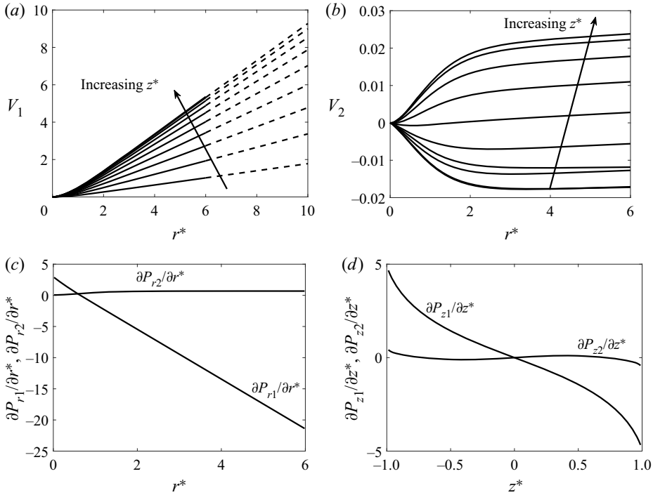
Figure 24. The variation of the functions (a) V_1 , (b) V_2 and (c) \partial P_{r1}/\partial r^* and \partial P_{r2}/\partial r^* with radial distance, and (d) \partial P_{z1}/\partial z^* and \partial P_{z2}/\partial z^* with vertical position. Panels (a) and (b) show different values of z^* from -0.9 to 0 , (c) are the midplane values and (d) are for the cylinder surface. The dashed lines in (a) are the functions V_{1\infty} .
