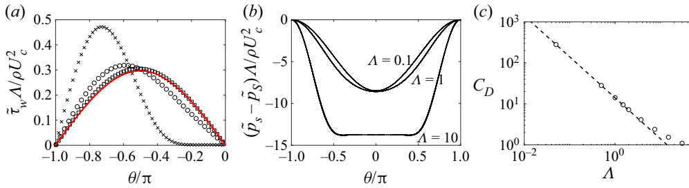
Figure 18. (a) The midplane friction coefficient for \Lambda = 0.1 ( \square ), 1 ( \circ ) and 10 ( \times ). (b) The pressure coefficient for \Lambda = 0.1 , 1 and 10. (c) Drag coefficient as a function of \Lambda ; the current numerical simulations are shown as circles, Lee & Fung's (1969) force expression for a Stokes flow past a cylinder is shown as a black dashed line and Thompson's analytical solution is given by the red line. All results are for \epsilon = 0.1 .
