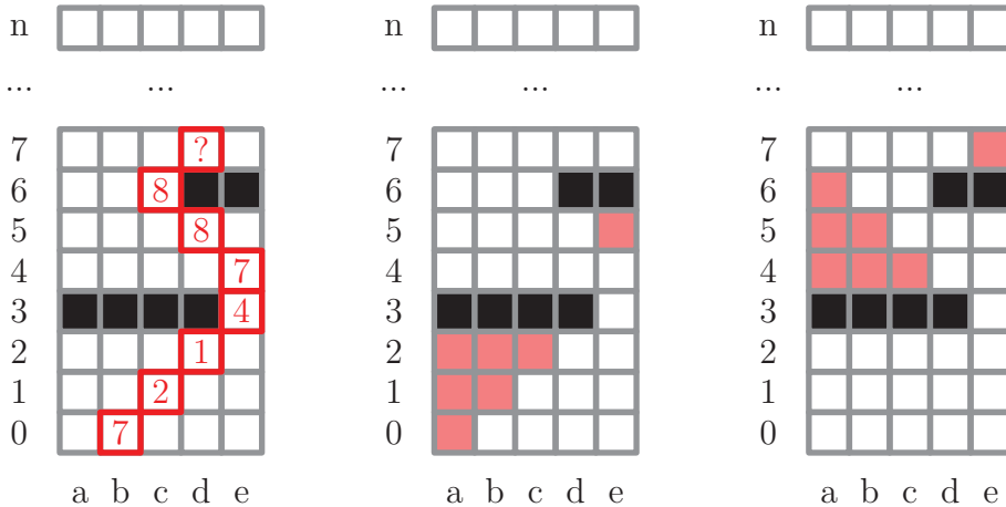
Fig. 2. Possible evolution starting from b (left), states from which less than three decision steps can be done (middle, pale red) and states that cannot be reached, no matter what the initial state at step 0 is and which controls are selected (right, pale red). The black squares represent unavailable columns: only e and a, b, c belong to State 3 and State 6 , respectively.
