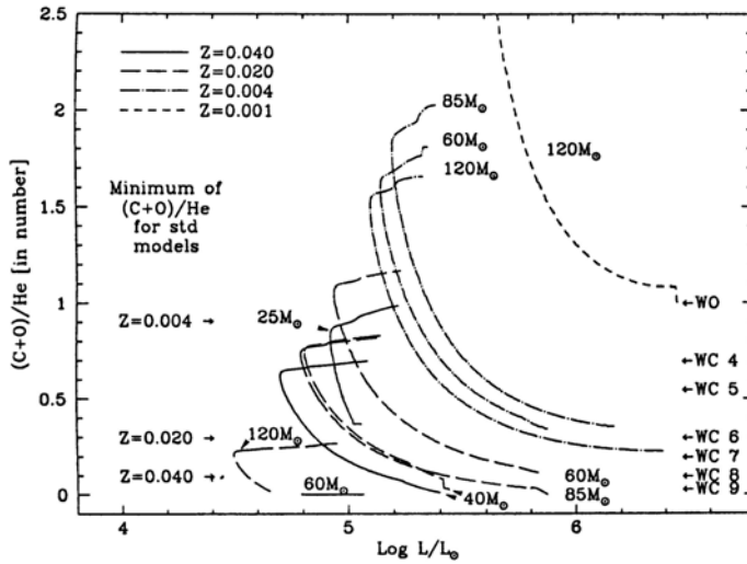
Figure 7. The (C+O)/He ratios in WC stars as a function of L for different Z and initial masses, cf. Maeder & Meynet (1994) and Meynet & Maeder (2005).
