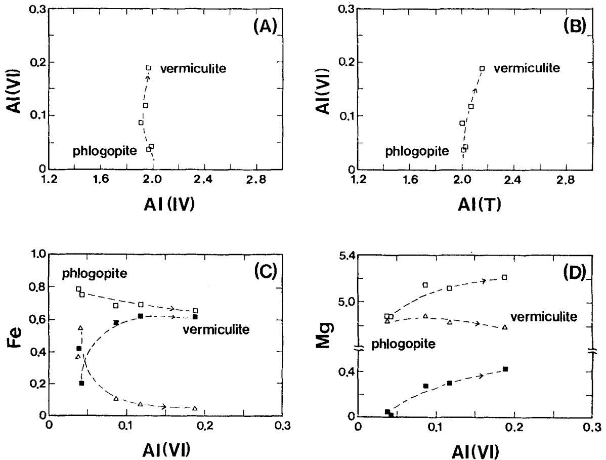
Figure 5. Compositional variations for phlogopite weathering to vermiculite: A) Al(IV) (tetrahedral Al) vs. Al(VI) (octahedral Al); B) Al(T) (total Al) vs. Al(VI); C) Al(VI) vs. Fe (open rectangle = Fe 2+ + Fe 3+ ; solid rectangle = Fe 3+ ; and open triangle = Fe 2+ ); and D) Al(VI) vs. Mg (open rectangle = total Mg; open triangle = Mg in octahedral sites assuming there are 0.2 vacancies per unit cell in octahedral sites; and solid rectangle = Mg treated as interlayer cations, assuming there are 0.2 vacancies per unit cell in octahedral sites).
