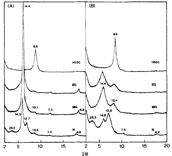
Figure 4. X-ray diffraction patterns of oriented, Mg-saturated, ethylene-glycolated, and heat-treated for some representative samples of <2 \mu\text{m} size fractions of vermiculite: A) vermiculite derived from phlogopite (P-3) and B) vermiculite derived from biotite (B-3). N = untreated, MG = Mg-saturated, EG = ethylene glycol saturated, and H550 = heated to 550°C. Numbers by peaks are angstroms (Å).
