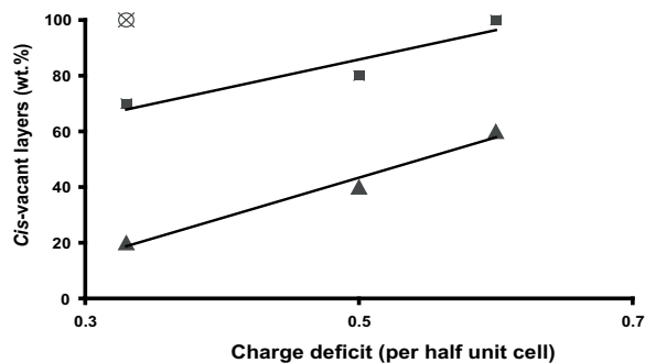
Figure 11. Evolution of the relative proportion of cis -vacant layers as a function of the layer charge deficit. \blacktriangle : SB (1,2 or 3) -280 samples; \blacksquare : SB (1,2 or 3) -325 samples; \circ : SB1-350; \times : (Klopprogge et al. , 1990).
