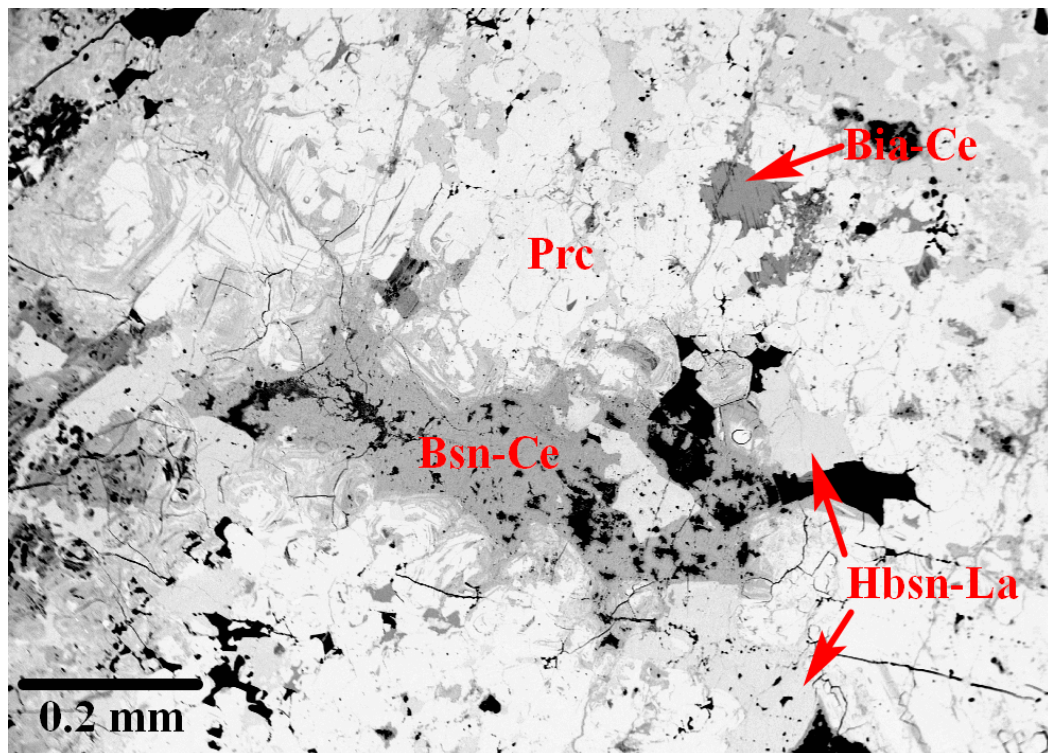
Figure 2. Hydroxylbastnäsite-(La) (Hbsn-La) grains in aggregate of other LREE minerals and quartz (black areas) from Mochalin Log. Prc – percleveite-(Ce) / percleveite-(La), Bsn-Ce – Ca-enriched variety of bastnäsite-(Ce), Bia-Ce – biraite-(Ce). Cotype specimen. Polished section, SEM (backscattered electron) image.
