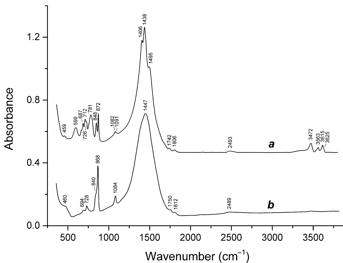
Figure 3. Powder infrared absorption spectra of (a) holotype hydroxylbastnäsite-(La) from Vuoriyarvi and (b) bastnäsite-(Ce) with the composition (\text{Ce}_{0.54}\text{La}_{0.26}\text{Nd}_{0.12}\text{Pr}_{0.06}\text{Sm}_{0.01}\text{Ca}_{0.01})_{\Sigma 1}(\text{CO}_3)\text{F}_{0.98}(\text{OH})_{0.01} from Mt. Ploskaya, Western Keivy, Kola Peninsula, Russia.
