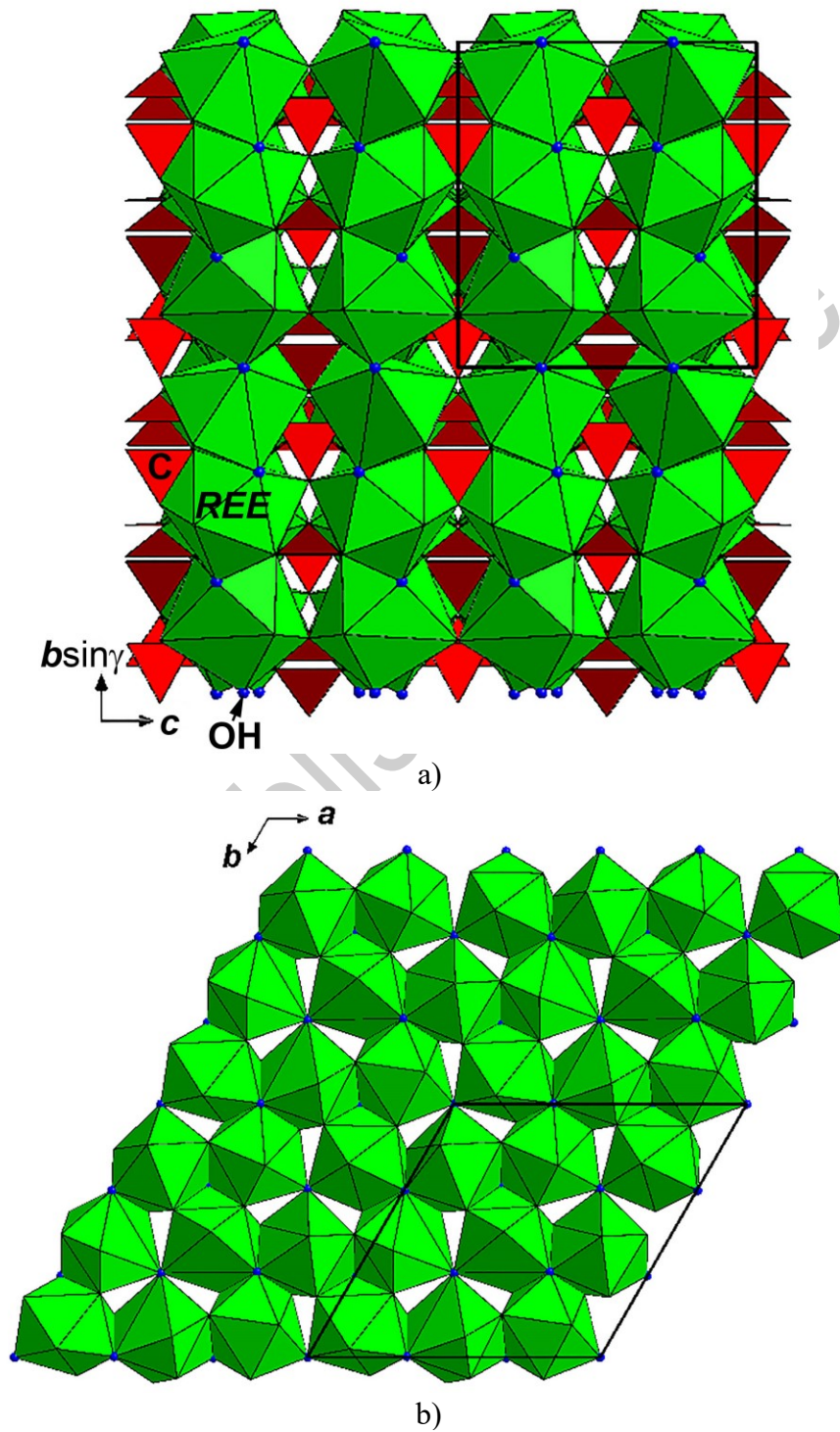
Figure 5. The crystal structure of hydroxylbastnäsite-(La) projected along the a axis (a) and the
