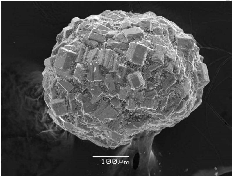
Figure 1. Clusters of hydroxylbastnäsite-(La) crystals from Vuoriyarvi. Holotype specimen. SEM (secondary electron) images.
