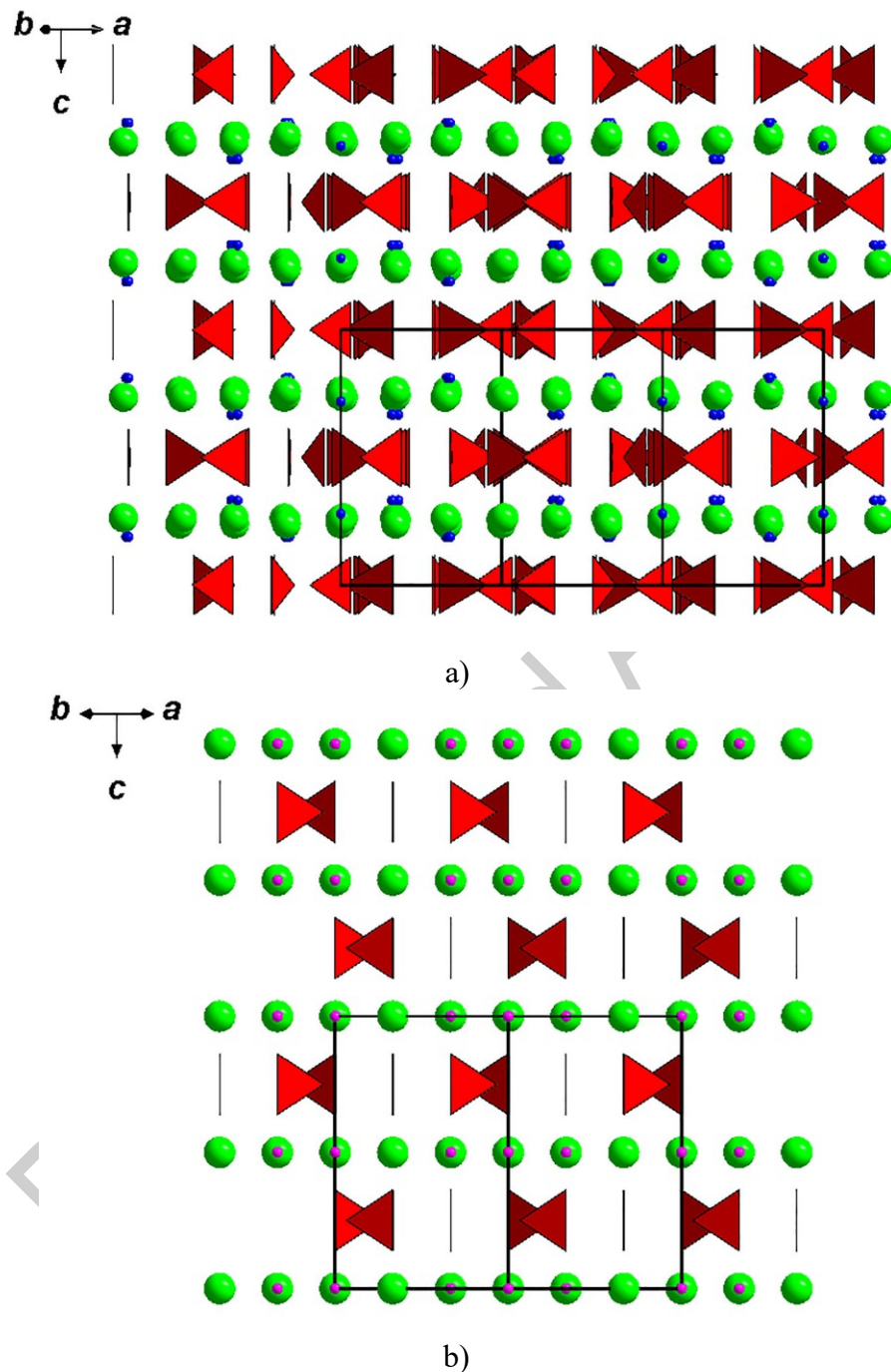
Figure 6. The crystal structures of hydroxylbastnäsite-(La) (projected along [120]; a) and bastnäsite-(Ce) (projected along [110]; b: drawn after Donnay and Donnay, 1953). For legend see Fig. 5; fluorine atoms in bastnäsite-(Ce) are shown as small reddish-pink circles. The unit cells are outlined.
