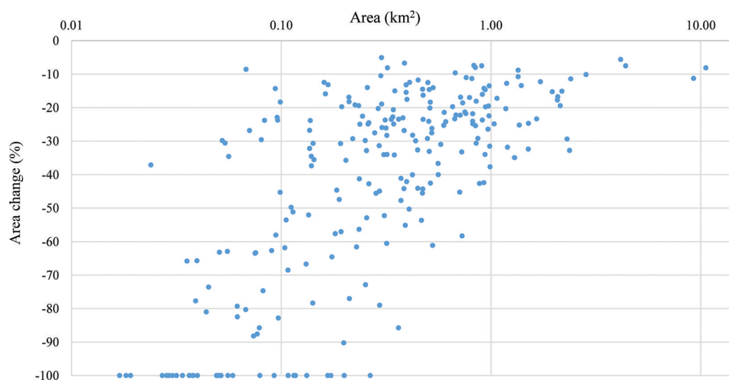
Fig. 5. Scatter plot of relative changes in glacier area vs initial glacier size for the 243 glaciers during 1989–2012.
