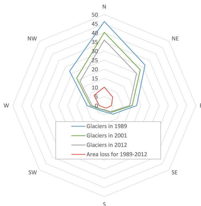
Fig. 4. Distribution of glacier areas and their changes according to aspect in the Karatal river basin during 1989–2012.
