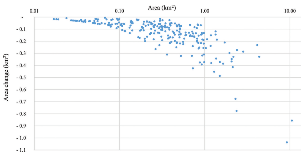
Fig. 6. Scatter plot of absolute changes in glacier area vs initial glacier size during 1989–2012.
