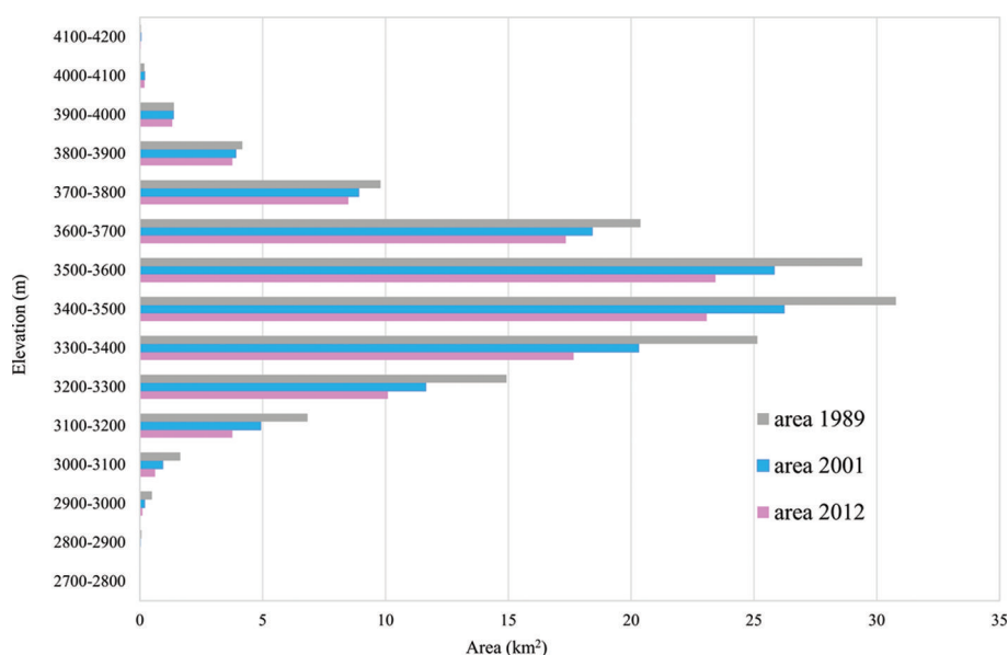
Fig. 7. Distribution of glacier areas and their changes vs elevation interval in the Karatal river basin.
