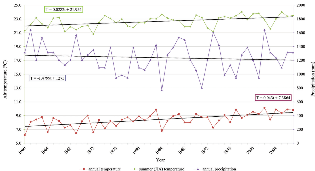
Fig. 8. Annual and summer (June–August (JJA)) temperature and annual precipitation at Taldykorgan station.
