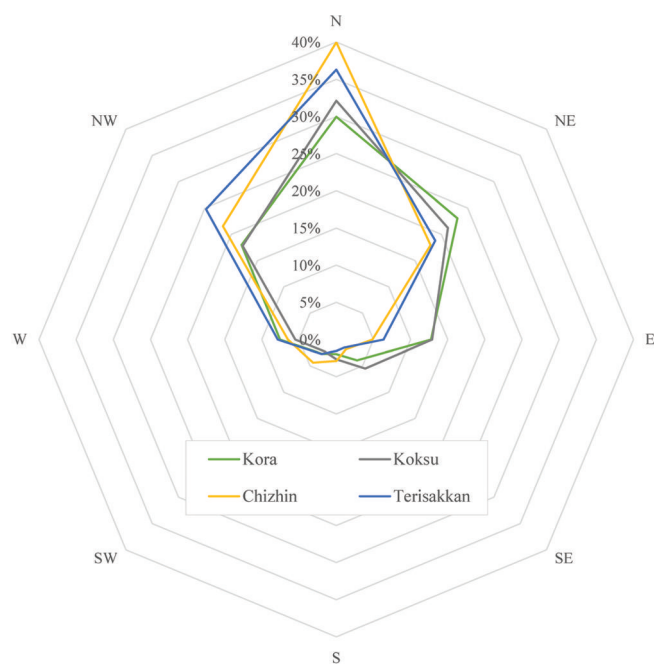
Fig. 3. Distribution of glacier areas according to aspect in different sub-basins during 1989–2012.
