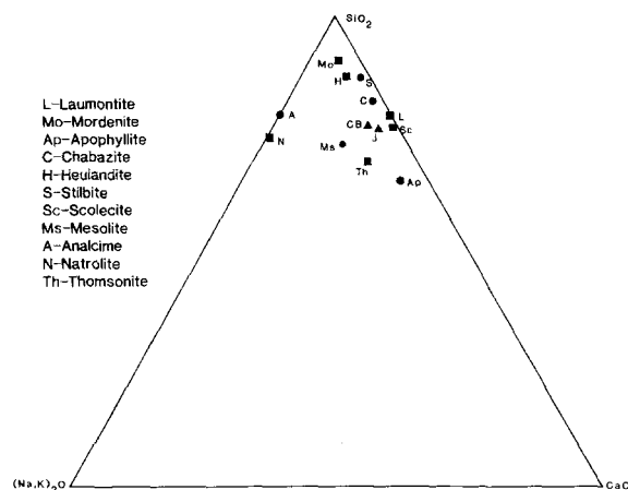
Figure 7. \text{SiO}_2 - (\text{K},\text{Na})_2\text{O} - \text{CaO} variation diagram of zeolites, apophyllite, and unaltered tholeiitic basalt in the Siletz River Volcanics. Circles represent minerals analyzed for this study (Table 1), squares are representative zeolite compositions, and triangles are unaltered basaltic lavas from Coffin Butte quarry (CB) and JayTe'el quarry (J) (Table 2).
