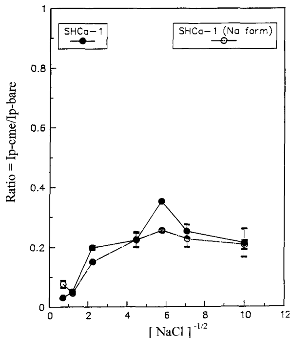
Figure 2. The ratio currents ( R = I_{p,CME}/I_{p,bare} ) for reduction of K_3Fe(CN)_6 at Ca-exchanged and Na-exchanged SHCa-1 modified electrodes as a function of the concentration of NaCl in the swelling solution.
