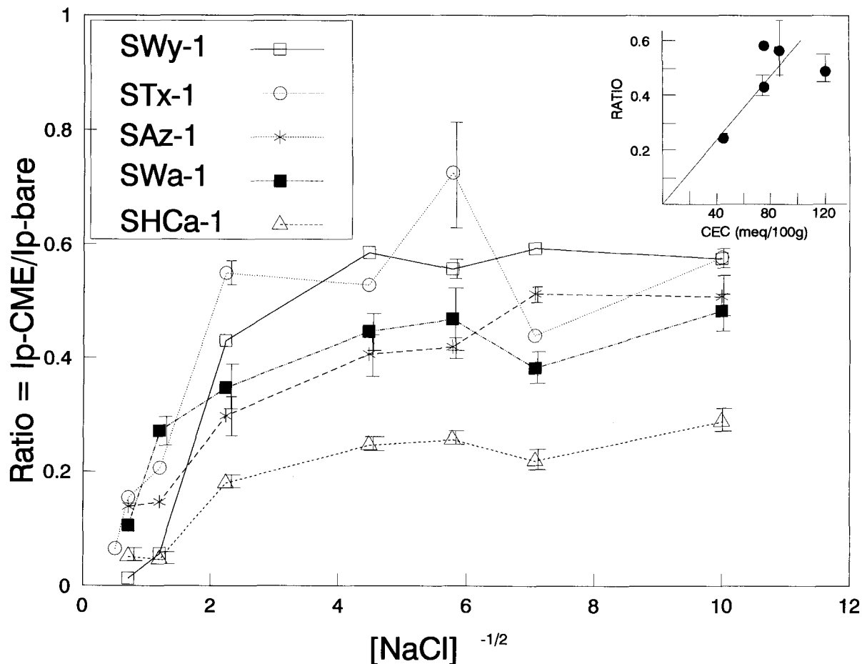
Figure 5. The ratio currents ( R = I_{p,CME}/I_{p,bare} ) for the reduction of \text{Na}_3\text{Fe}(\text{CN})_6 at variable clay-modified electrodes as a function of NaCl in the swelling solution. Inset shows R at 0.02 M NaCl as a function of the cation exchange capacity (CEC) of the clay.
