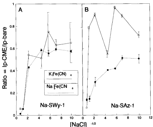
Figure 4. The ratio currents ( R = I_{p,CME}/I_{p,bare} ) for the reduction of Fe(CN)_6^{3-} at A) Na-SWy-1 and B) Na-SAz-1 as a function of NaCl in the swelling solution. Upper curve is K_3Fe(CN)_6 . Lower curve is Na_3Fe(CN)_6 .
