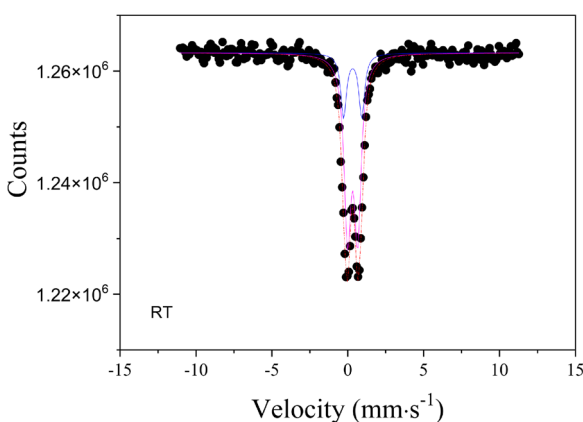
Fig. 5 Mössbauer spectrum for the synthesis product with (\text{Fe}/\text{Si})_{\text{ini}} = 0.75 at 290 K
