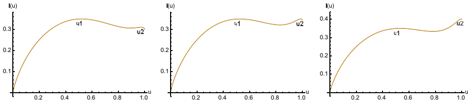
FIGURE 3. Three plots of l_\theta(u) for k = 7 and \theta = 0.3 , \theta = \hat{\theta}(7) , and \theta = 0.4 . For \theta = 0.3 , u_1^*(\theta) is the global maximiser; for \theta = \hat{\theta}(7) , u_1^*(\theta) and u_2^*(\theta) are both global maximisers; and for \theta = 0.4 , u_2^*(\theta) is the global maximiser. In the figures, the function l_\theta(u) is denoted by l(u) and the local maximisers u_1^*(\theta) and u_2^*(\theta) are denoted by u1 and u2 respectively. The BEE-phase is (u_1^*(\hat{\theta})^k, u_2^*(\hat{\theta})^k) .
