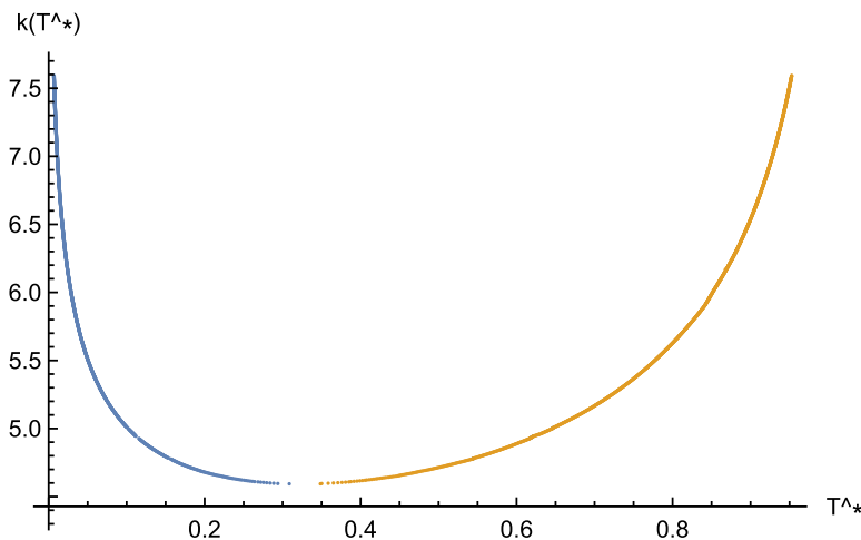
FIGURE 1. A numerical picture of the phase diagram. The left and right lines together form the critical curve (T^*, k_c(T^*)) . In the figure, T^* is denoted by T^* and k_c(T^*) is denoted by k(T^*) . The minimum is achieved at k_0 = 4.591 \dots and T_0 = 0.3237 \dots
