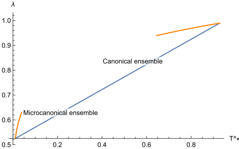
FIGURE 2. A numerical picture of the average largest eigenvalue \lambda = \lim_{n \rightarrow \infty} \frac{1}{n} \mathbb{E}[\lambda_n] of the adjacency matrix under the microcanonical ensemble (top curve) and the canonical ensemble (bottom curve), as a function of T^* for a subgraph F with k = 7 edges and maximum degree d = 5 . The top curve is shown only for T^* in the replica symmetric region. In the region of replica symmetry breaking we have no explicit expression for \lambda under the microcanonical ensemble.
