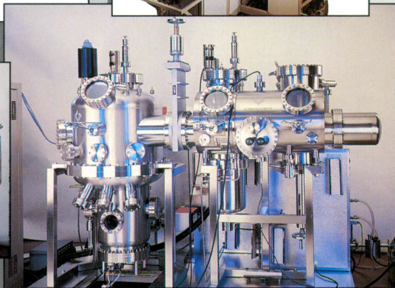
Research UHV for evaporation onto heated 6" wafers
