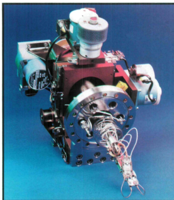
Fully motorized 5-axis HPT high precision manipulator
