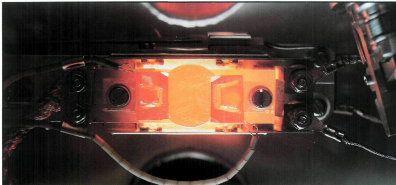
An LN 2 cooled HPT manipulator operating at high temperature
