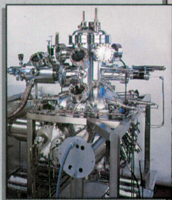
Research UHV for thin film high T_c superconductors
