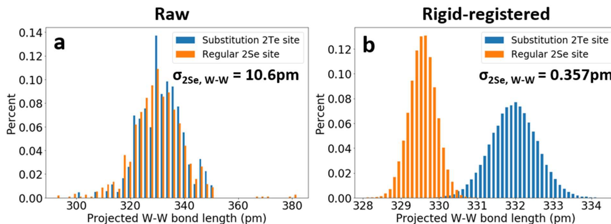
Figure 2. Distribution of projected W-W bond length measurements of \text{WSe}_{2-x}\text{Te}_x for (a) raw (b) rigid-registered images. Unlike in the raw data, the rigid-registered images show well-separated distributions of bond length measurements on regular and defect-containing (2Te-substituted) sites. The measured bond length of 2Te-substituted site is 332.0 \pm 0.61 pm, and 329.6 \pm 0.36 pm for the regular 2Se site. We are able to improve our precision by factor of 30 after aligning and summing images of 2Te (183 images) and 2Se (523 images) sites respectively. With these methods, we were able to measure the local strains in 2D materials induced by individual atomic substitutions with sub-picometer precision for the first time.
