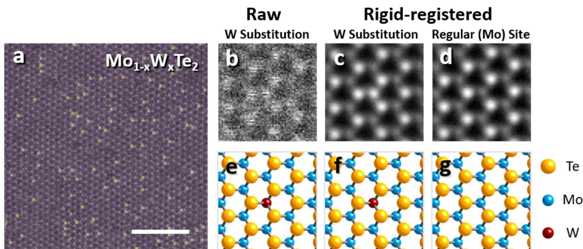
Figure 1. Identification of W substitutions using deep learning on a STEM image of \text{Mo}_{1-x}\text{W}_x\text{Te}_2 (a) annular dark-field STEM image of \text{Mo}_{1-x}\text{W}_x\text{Te}_2 , overlaid with CNN determined positions of W substitutions in yellow and regular lattice sites in purple. Scale bar is 2.5 nm. (b-d) Raw and summed images generated from (a) and (e-g) corresponding cartoons of regular Mo and W-substituted lattice sites. By aligning and summing 274 equivalent lattice positions, we produce rigid-registered images (c-d) with 15 times higher SNR than the raw image (b). Image widths in (b-d) are 1.3 nm.
