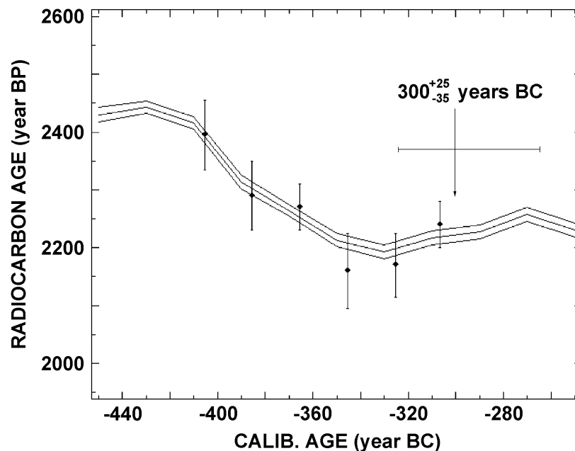
Figure 2 Results of the ^{14}\text{C} age measurements of D-5 sample of Pazyryk barrow 2 (Le-5558–Le-5563). The log was split in 6 pieces, and each included 20 tree rings. To determine the absolute age of sample the data of ^{14}\text{C} age were compared to the bidecadal calibration curve (Pearson and Stuiver 1993; Stuiver and Pearson 1993). The position of experimental points relative to the calibration curve was determined by means of minimization of \chi^2 statistics (Zaitseva et al. 1998). According to our estimation the construction date of Pazyryk barrow 2 was about 300 BC with error 25–35 yr ( 2\sigma ).
