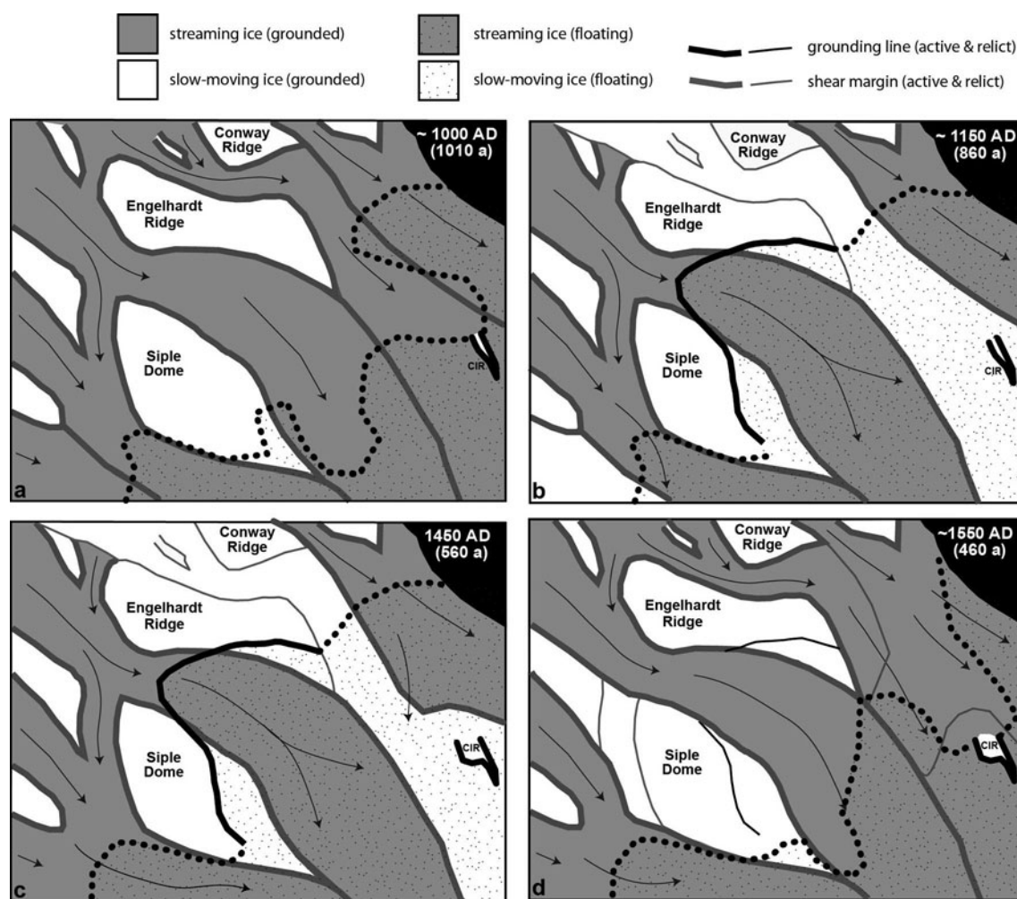
Fig. 2. Changes in the Siple Coast ice streams from (a) AD 1000 to (b) AD 1150 to (c) AD 1450 to (d) AD 1550. Fast-moving ice is colored dark gray, slow-moving ice is white and floating ice is overlaid with dots. Lines denote ice-dynamic boundaries, shear margins and grounding lines; known position is given as a solid line, and unknown is dotted. Active boundaries are plotted with thick lines, and inactive boundaries marking the presence of a modern-day surface scar are shown as thin lines. Arrows indicate flow direction and migration direction of margins.
