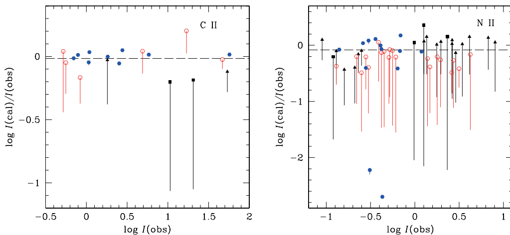
Figure 1. Comparison of calculated and observed line intensities of C II and N II. Lines from s states: black squares, p states: black triangles, d states: red circles, f and g states: blue filled circles. The dashed line is the average I(\text{calc})/I(\text{obs}) . Vertical lines show the increase of intensity due to fluorescence excitation (colour on line).
