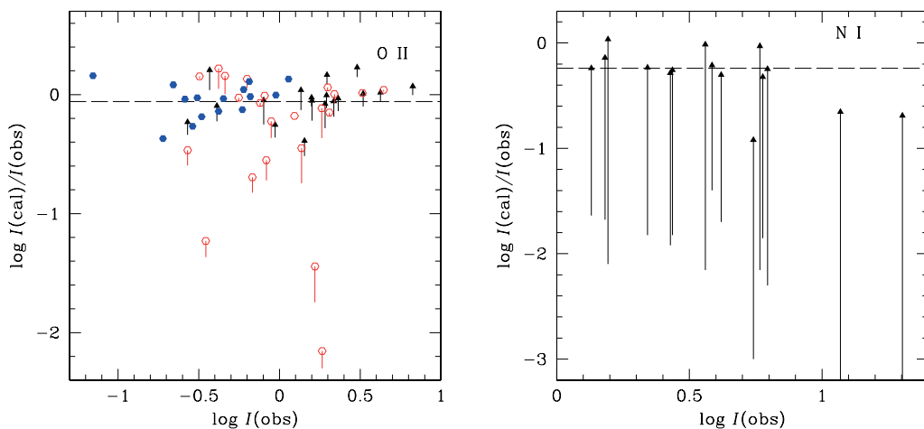
Figure 2. Same as figure 1 for O II and N I (colour on line).
