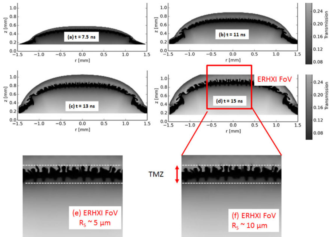
Figure 10. (a) to (d) Postprocessed radiographs of RTI multimode evolution with a titanium backlighter according to ERHXI spatial resolution of 10\ \mu\text{m} . (e) and (f) Comparison of ERHXI field of view with spacial resolution of 5\ \mu\text{m} and 10\ \mu\text{m} . The tips of the spikes are better resolved in (e). The turbulent mixing zone width is defined as the average distance between the RTI spike and bubbles.
