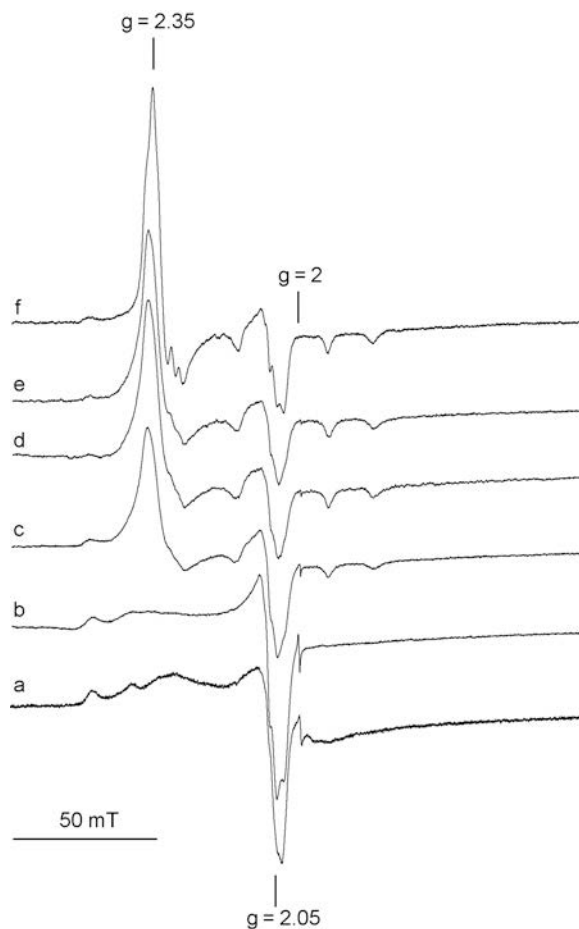
Figure 10. EPR spectra of the hydrothermally treated sample Cu 150 after stepwise heating at 400°C (a), 600°C (b), 625°C (c), 650°C (d), 700°C (e), and 1000°C (f).
