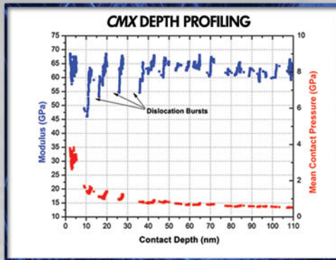
Coupled AC/DC force modulation for quantitative nanoscale dynamic characterization from the initial surface contact.
