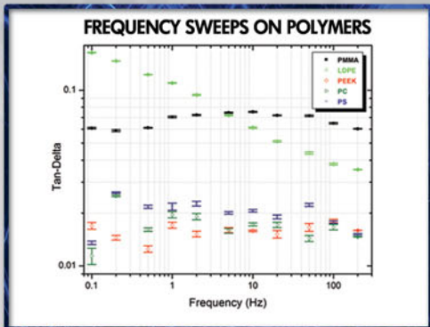
High bandwidth electronics for enhanced dynamic characteristics and dynamic testing range (0.1Hz - 300Hz).
