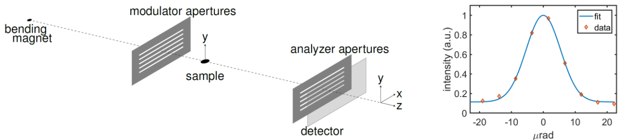
Figure 1. Sketch of the experimental setup, the white beam from bending magnet is amplitude-modulated before it reaches the sample and it is analyzed by a set of aperture before detection. The experimental illumination function of such a system is reported in the panel on the right-hand side.
