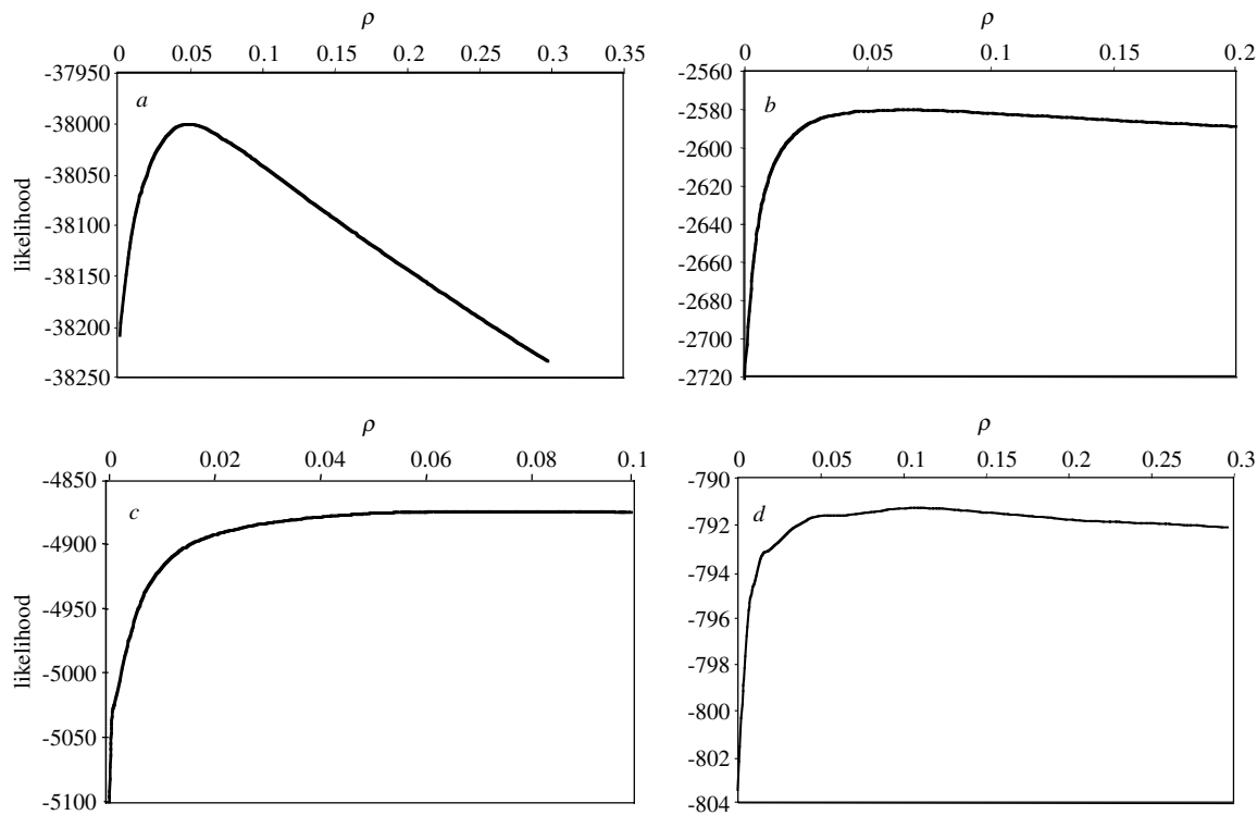
Fig. 4. Likelihood curves for estimation of \rho for four data sets produced by Ldhat. (a) Agph-DABI ; (b) 40 kb locus; (c) Mhc -linked loci (40 kb, DAB3 , DAB1 promoter); (d) \beta -actin ( BACT2 ). The shape of the curve for \beta -fibrinogen ( BFIB7 ) was very similar to that in (d).
