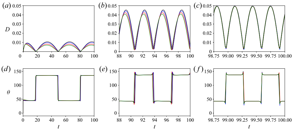
Figure 6. Droplet deformation, D , and inclination angle, \theta , over time for the external magnetic field in the z -direction as a function of oscillatory shear frequency and Ca_{mag} . First column for \omega = 0.10 , second for \omega = 1.00 and the last one for \omega = 10.00 . Black lines represent the flow in the absence of magnetic field, blue lines refer to Ca_{mag} = 4.00 , red to Ca_{mag} = 10.00 and green to Ca_{mag} = 16.00 .
