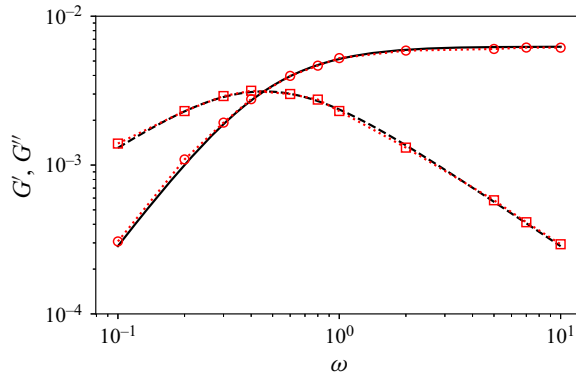
Figure 2. Elastic, G' , and loss, G'' , moduli as a function of the non-dimensional angular frequency, \omega . Red circles and squares represent, respectively, our results for G' and G'' . The solid and dashed black lines refer to Palierne’s model (Palierne 1990).
