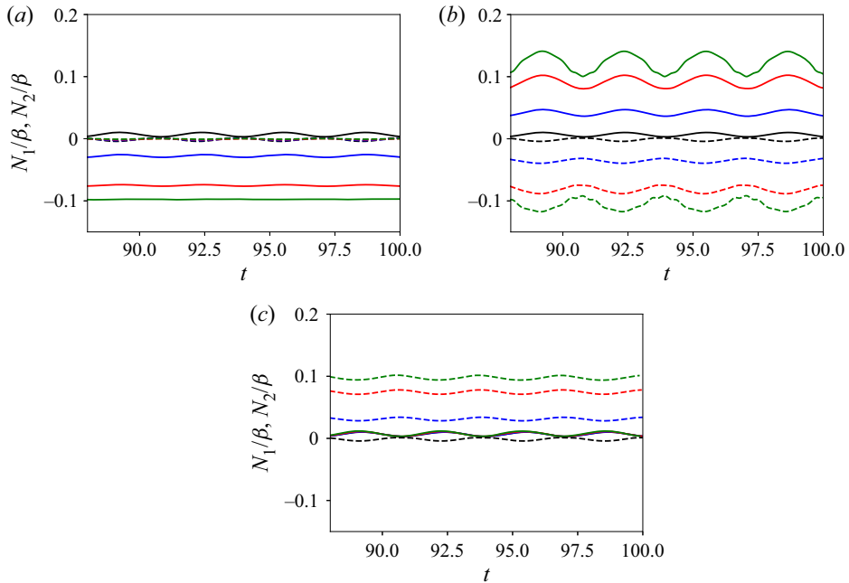
Figure 9. First (solid lines) and second (dashed lines) normal stress differences, scaled by the volume fraction, for an external magnetic field in the x (a), y (b) and z (c) directions and \omega = 1.00 . Black, blue, red and green colours are, respectively, for Ca_{mag} = 0, 4, 10 and 16 .
