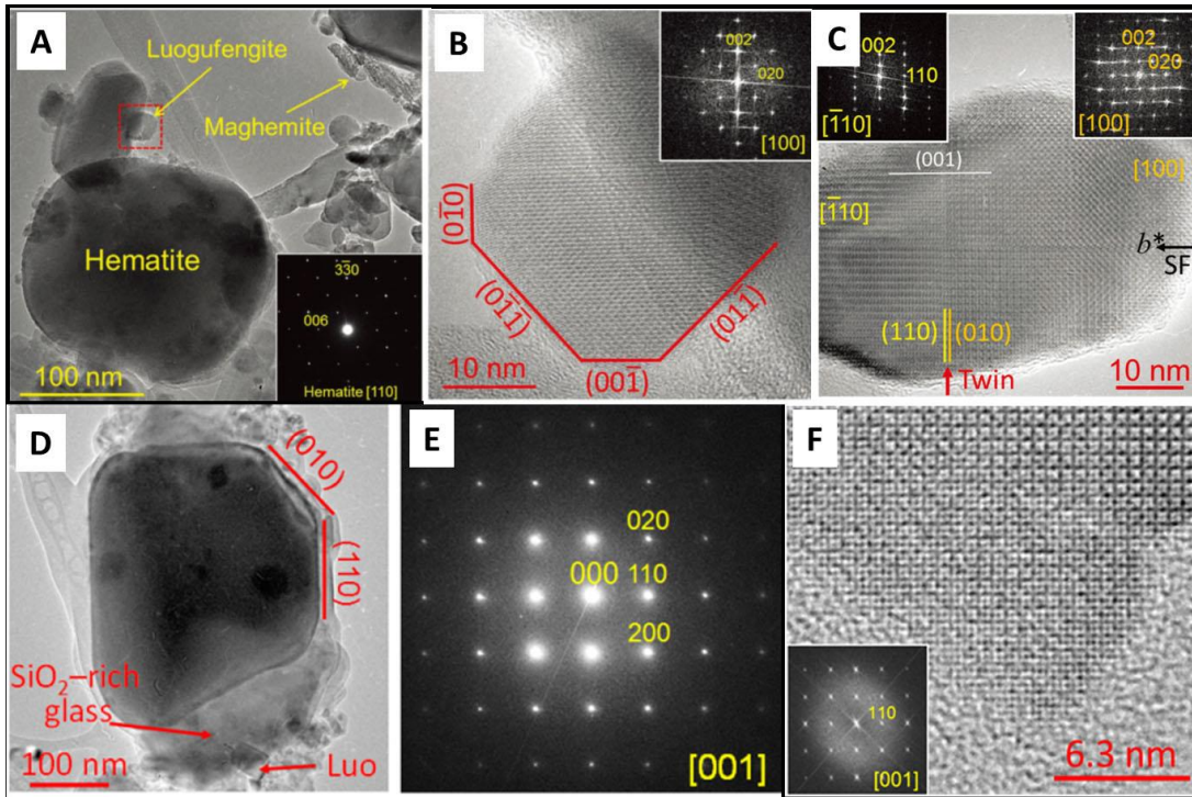
Figure 1. Bright-field TEM images, SAED, and High-resolution TEM, FFT patterns of (A-C) luogufengite and (D-F) valleyite.
