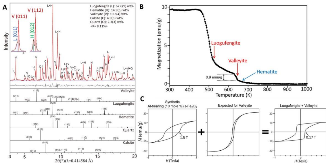
Figure 2. (A) Synchrotron X-ray diffraction pattern of a treated sample (B) Temperature dependence of magnetization of the luogufengite and valleyite. (C) Hysteresis loops of synthetic Al-bearing \epsilon\text{-Fe}_2\text{O}_3 , expected valleyite, and natural luogufengite/valleyite sample.
