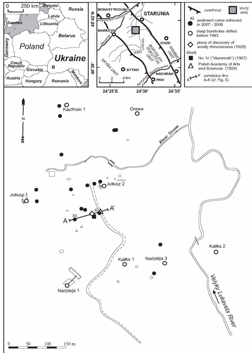
Figure 1 Sketch map of the Starunia paleontological site (Carpathian region, Ukraine) showing locations of the discovery of woolly rhinoceroses and that of boreholes from which microfossils were extracted from sediment cores for ^{14}\text{C} dating.
