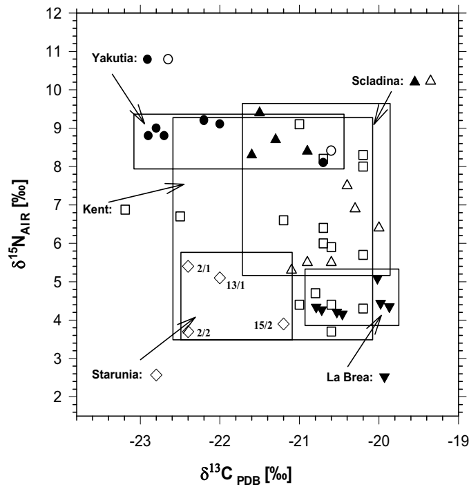
Figure 3 Relationship between \delta^{15}\text{N} and \delta^{13}\text{C} values of collagen extracted from 4 samples (2 bones and 2 teeth) representing woolly rhinoceros remnants found in the Starunia area, Ukraine (symbols indicate no. of sample), compared to other data of rhinoceroses and mammoths from different locations in North America, Europe, and Asia: La Brea (Coltrain et al. 2004); Kent (Bocherens et al. 1995); Scladina Cave (Bocherens et al. 1997); and Yakutia (Bocherens et al. 1996). Rhinoceroses = open symbols; mammoths = filled black symbols. Numbers next to the symbols of Starunia samples correspond to numbers listed in Table 3.
