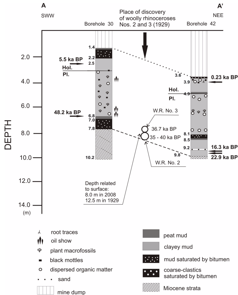
Figure 5 Lithological structure of Quaternary sediments in the immediate surroundings of the discovery site of woolly rhinoceroses remnants in the Starunia area. Shown are 2 sediment profiles (borehole 30 and 42, cf. Figure 1). The dashed line shows schematically the present position of the top of Miocene strata, whereas the dotted line represents the bottom of the mine dump along the A-A' cross-section. Position of 14 C-dated macrofossils retrieved from the sediment cores is marked by horizontal arrows: W.R. – woolly rhinoceros; PI. – Pleistocene; Hol. – Holocene.
