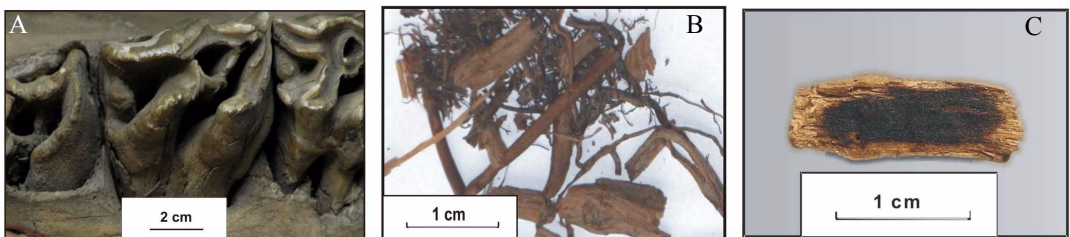
Figure 2 A) Dated teeth of rhinoceros No. 3 (lower jaw); B) Macrofossils retrieved from sediment cores in the Starunia area representing different types of plant material. The sample composed mostly of tiny fragments of green plants; C) Piece of wood with hydrocarbon contamination still visible (dark inner part) after procedure of chemical cleaning.
