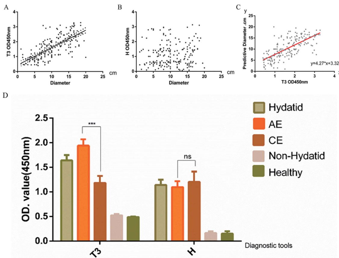
Figure 4. OD450 nm results of the new recombinant antigen T3 and commercial H reagent ELISA. The abscissa was the diagnostic reagent, and the ordinate was the OD value, P < 0.0001 (***) (A) There was a linear relationship between lesion diameter and OD value in T3 group, r = 0.707 ; (B) Commercial H reagents had no linear relationship; (C) Regression model for predicting lesion diameter using T3 OD value. Y axis, predicted diameter (cm), X axis, OD value. (D) The OD value of AE was significantly higher than that of CE, while the OD value of AE and CE determined by H reagent showed no significant difference. (ns), the small plot was the 95% confidence interval.
