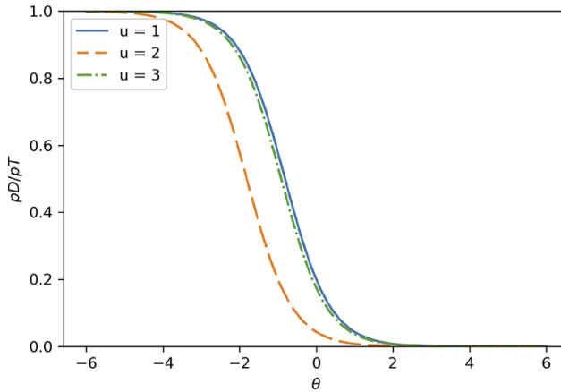
Figure 3. \frac{\bar{p}_D(\theta, u)}{p_T(\theta, u)} when \sigma = 1.7, b = 0.0, \gamma_2 = 1, \gamma_3 = 0.1, K = 4 .
