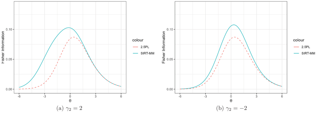
Figure 7. Fisher information of SIRT-MM models with a = 0.75, b = 0, \gamma_3 = 0, K = 4 , and different \gamma_2 ; and the corresponding 2.5PL models with \gamma_1 = 0 .
