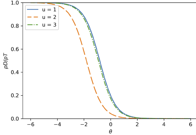
Figure 3. \frac{\bar{p}_D(\theta, u)}{p_T(\theta, u)} when a = 1.7, b = 0.0, \gamma_2 = 1, \gamma_3 = 0.1, K = 4 .
