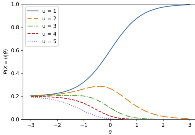
Figure 1. Item category response function: a = 1.7, b = 0.0, K = 5 .
