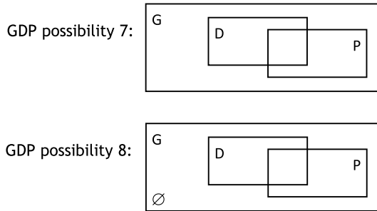
Figure 3. The progressive GDP possibilities 7 and 8; \emptyset is the empty set, such that G = D \cup P for possibility 8.
