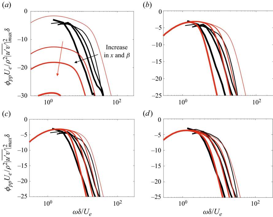
Figure 10. Comparison between model predictions of (5.2) with progressive changes described in text (—, red solid line) and Wu & Piomelli (2018) (—, thick solid line) data in attached flows with weak to strong APGs, to show improvement brought by each model change. (a) The Goody (2004) model (predictions are plotted using the optimal normalizations), (b) pressure scale changed from \tau_w to \rho |u'v'|_{max} , (c) additionally replacing dependency on R_r with that on y_w^+ , (d) further addition of Coles' parameter. Thicker lines indicate increase in x (corresponding to increasing \beta ).
