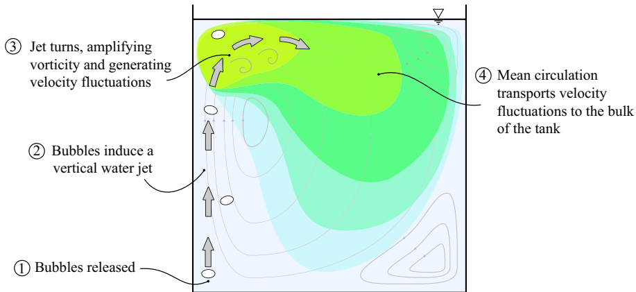
Figure 9. A schematic diagram showing the mechanism proposed for the observed transition. Arrows represent the impinging jet of rising fluid, and coloured regions schematically represent areas with varying intensities of velocity fluctuations with intensity decreasing from yellow to light blue.
