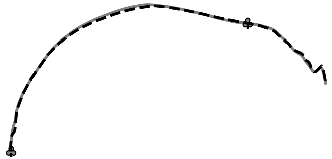
Fig. 10. Surface evolutions computed using different SIA formulations, after t = 400 years. The horizontal mesh size is \Delta x = 2472 m. The time steps take the largest feasible values for the given mesh sizes (see Figure 9).
