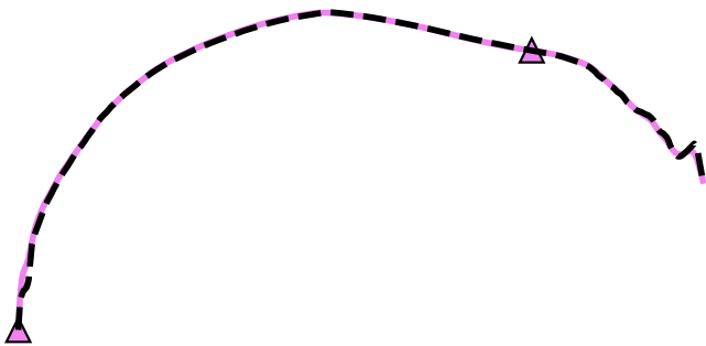
Fig. 10. Surface evolutions computed using different SIA formulations, after t = 400 years. The horizontal mesh size is \Delta x = 2472 m. The time steps take the largest feasible values for the given mesh sizes (see Figure 9).
