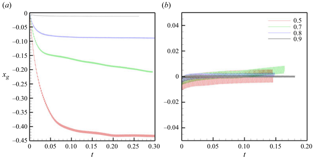
Figure 2. Evolution of the bubble centre of mass ( x_g ) for different dimensionless bubble radii R/R_c in SF 6 at A_c = 0.0667 , \Omega = 3.6 \times 10^3 : (a) \phi = 0 , (b) \phi = \pi/2 .
