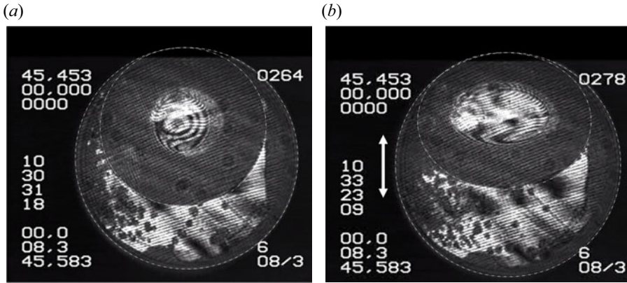
Figure 7. An SF 6 bubble (underlined by interrupted circle or ellipse) for (T - T_c) = -113 mK and R/R_c = 0.75 . (a) At equilibrium, (b) submitted to a harmonic vibration with frequency 1.6 Hz and amplitude 0.8 mm; double arrow indicates the vibration direction – experiment in MIR station carried out in parallel with the study by Garrabos et al. (2007). With the courtesy and permission of D. Beysens.
