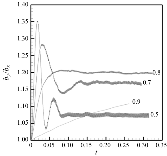
Figure 5. Evolution of the aspect ratio b_y/b_x of the bubble (assimilated to an ellipse), for different R/R_c . Fluid SF 6 , \phi = 0 , A_c = 0.0667 , \Omega = 3.6 \times 10^3 .
