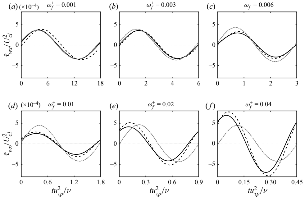
Figure 7. Single-period time evolution of the periodic streamwise wall stress \tilde{\tau}_{wx} for several forcing frequencies, \omega_f^+ = 0.001, 0.003, 0.006, 0.01, 0.02, 0.04 (plots (a–f), respectively). Line types correspond to LES using the MTS wall model (thick solid black), LES using the EQWM (thick dashed-dot grey), and DNS from Weng et al. (2016) (thick dashed black). The phase within the cycle is based on the imposed forcing frequency.
