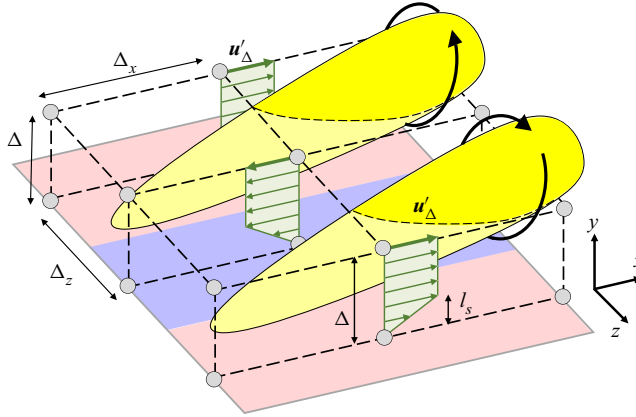
Figure 3. A schematic of the turbNEQ velocity profiles resulting from two counter-rotating wall-attached eddies. Circles indicate the LES grid points, and the blue surface indicates a possible region of negative velocity fluctuation (green arrows) induced between wall-attached eddies (yellow) that can be only partially resolved on the LES resolution.
