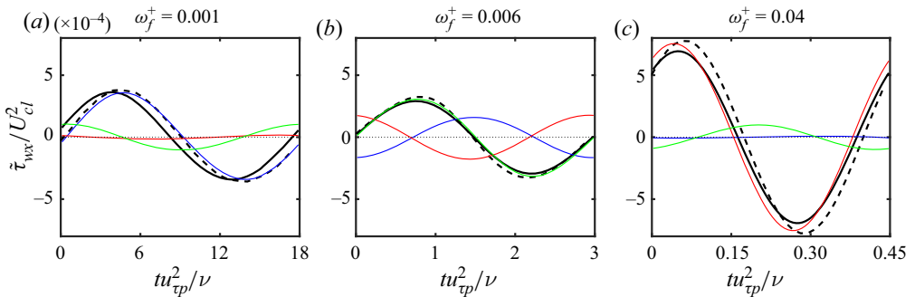
Figure 8. Single-period time evolution of the periodic streamwise wall stress \tilde{\tau}_{wx} for low, intermediate and high forcing frequencies: \omega_f^+ = 0.001, 0.006, 0.04 (plots (a–c), respectively). Line types correspond to LES using the MTS wall model (thick solid black), with LaRTE (thin solid blue), lamNEQ (thin solid red) and turbNEQ (thin solid green) parts, and DNS from Weng et al. (2016) (thick dashed black). The phase within the cycle is based on the imposed forcing frequency.
