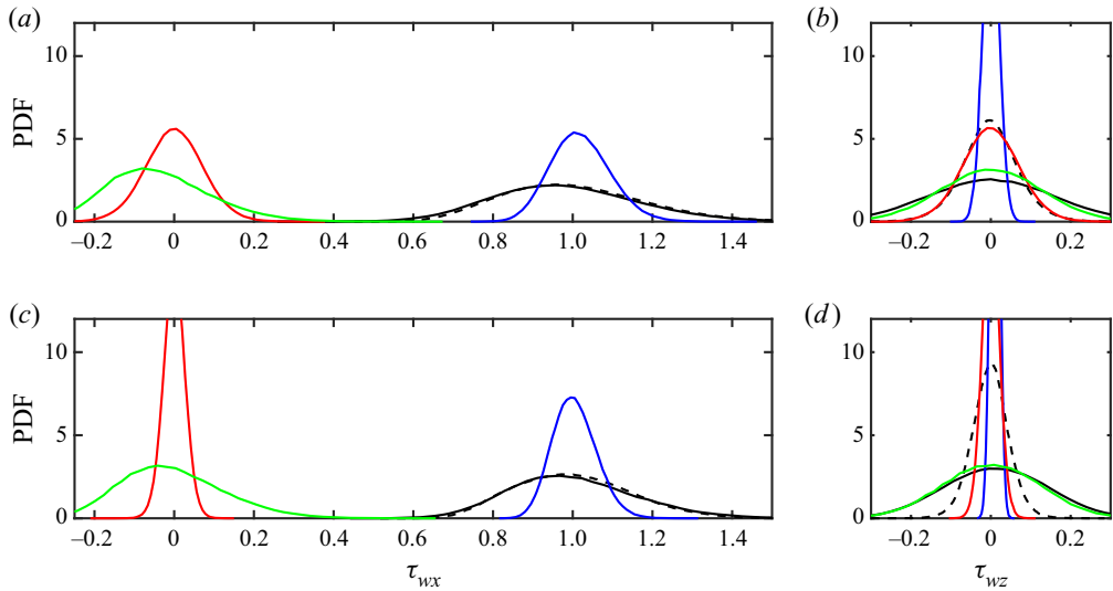
Figure 26. PDFs for \tau_{wx} and \tau_{wz} , for (a,b) Re_\tau = 1000 , and (c,d) Re_\tau = 5200 . The PDF curves correspond to the filtered DNS (dashed black lines), the LaRTE model (blue lines), the lamNEQ model (red lines), the turbNEQ term (green lines) and the MTS model (solid black lines). DNS data are obtained from the Johns Hopkins Turbulence Database (Graham et al. 2016; JHTDB 2021). The DNS PDFs are obtained from the Gaussian filtered wall stress where the filtering size is the same as the LES mesh size in the horizontal directions.
