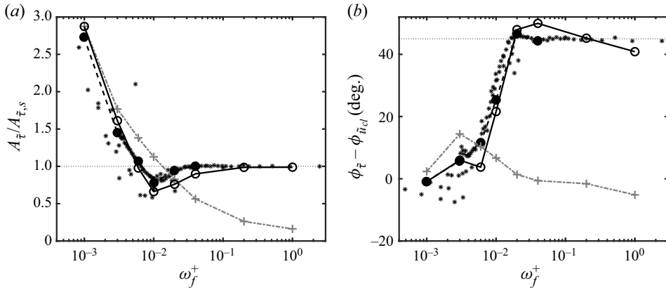
Figure 9. (a) The periodic wall-stress amplitude normalized by the Stokes solution amplitude. (b) The periodic wall-stress phase relative to the centreline velocity phase. Asterisks correspond to outside experimental, LES or DNS data from Ronneberger & Ahrens (1977) (experimental), Tardu et al. (1994) (experimental), Scotti & Piomelli (2001) (LES) and Weng et al. (2016) (DNS). The DNS data of Weng et al. (2016) are emphasized with filled circles and connected with thick dashed black lines. LES using the MTS wall model are shown with open circles and connected with thick solid black lines. LES using the EQWM are shown with plus symbols and connected with thick dashed-dot grey lines. The thin dotted horizontal black lines correspond to the Stokes solution.
