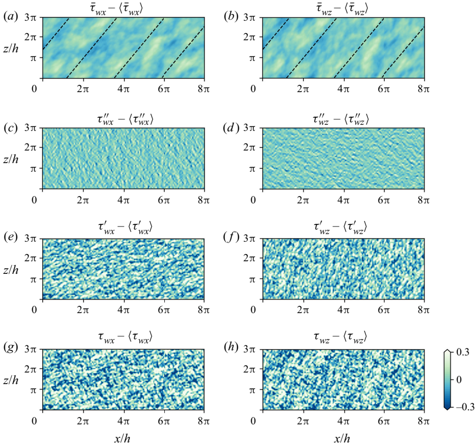
Figure 29. Contour plots of the wall-stress fluctuations (both streamwise and spanwise directions) for each component in the MTS wall model after the SSPG is applied at tu_{\tau_p,i}/h = +2.22 . These components include (a,b) LaRTE, (c,d) lamNEQ, (e,f) turbNEQ, and (g,h) the total MTS wall stress. The dashed lines in (a,b) represent the total wall-stress angle. Angled brackets represent averaging over the horizontal plane. An animation of the wall-stress evolution before ( t < 0 ) and after ( t > 0 ) the SSPG can be seen at https://www.cambridge.org/S0022112023005852/JFM-Notebooks/files/Figure-29/sspg_ws_contour_animation.html . The corresponding source code can be found at https://www.cambridge.org/S0022112023005852/JFM-Notebooks/files/Figure-29/sspg_ws_contour_animation.ipynb .
