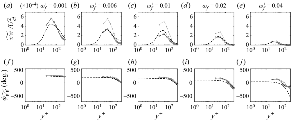
Figure 14. (a–e) Amplitude and (f–j) phase lead of \widetilde{v'v'} for five forcing frequencies, \omega_f^+ = 0.001, 0.006, 0.01, 0.02, 0.04 . Line types are the same as in figure 12.
