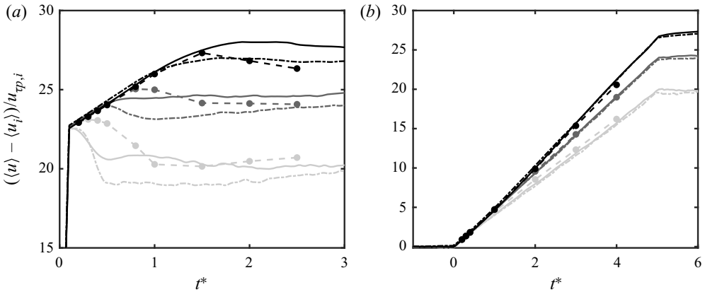
Figure 22. Time signals of the velocity perturbation (from the initial condition) at several heights for (a) T^* = 0.1 and (b) T^* = 5.0 . From light to dark lines, the heights correspond to y/h = 0.167, 0.5, 0.967 , which are the third, eighth and centreline LES grid points, respectively. The DNS (from Jung & Kim 2017), the LES with the MTS wall model, and the LES with the EQWM correspond to dashed lines with filled circles, solid lines, and dashed-dot lines, respectively. The circles correspond to the sample times given for the DNS.
