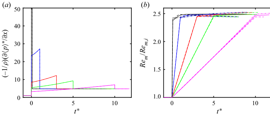
Figure 17. Time signals of (a) the pressure gradient forcing, and (b) the mean Reynolds number ( Re_m = 2hU_m/\nu ) divided by the initial mean Reynolds number, Re_{m,i} , for different acceleration ramp rates. Ramp rates T^* = 0.1, 1.0, 3.0, 5.0, 10.0 correspond to black, blue, red, green and magenta lines, respectively. Line types for the DNS of Jung & Kim (2017), LES with the MTS wall model, and LES with the EQWM are dashed, solid and dashed-dot, respectively.
