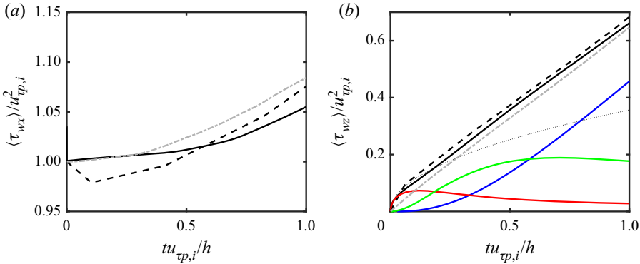
Figure 28. (a) Streamwise and (b) spanwise wall stress after a suddenly applied spanwise pressure gradient. Line types correspond to the DNS of Lozano-Durán et al. (2020) (thick dashed black lines), LES with the EQWM (dashed-dot grey lines), and the total wall stress for LES with the MTS wall model (solid black lines). In (b), wall stresses for the LaRTE, lamNEQ and turbNEQ components of the MTS wall model are shown with blue, red and green lines, respectively. The thin dotted line in (b) corresponds to the Stokes solution wall stress. Angled brackets represent ensemble averaging over the horizontal plane and over five independent simulations.
