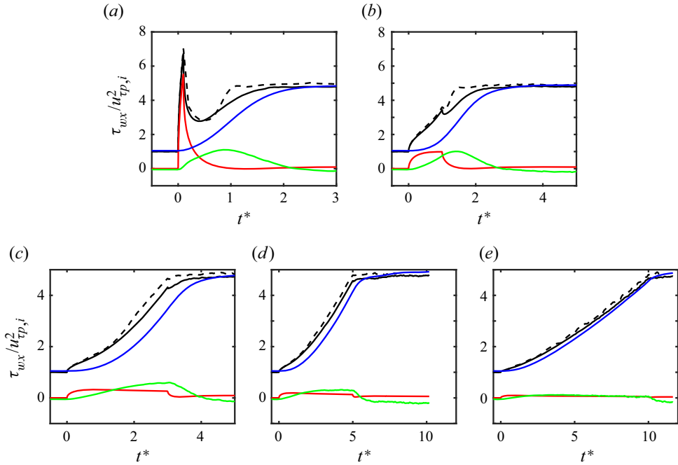
Figure 20. Time signals of the wall stress for different acceleration ramp rates. Ramp rates T^* = 0.1, 1.0, 3.0, 5.0, 10.0 correspond to plots (a–e), respectively. The curves compared are the DNS of Weng et al. (2016) (thick dashed black line) and the LES with the MTS wall model (thick solid black line), with LaRTE (thick blue line), lamNEQ (thick red line) and turbNEQ (thick green line) components.
