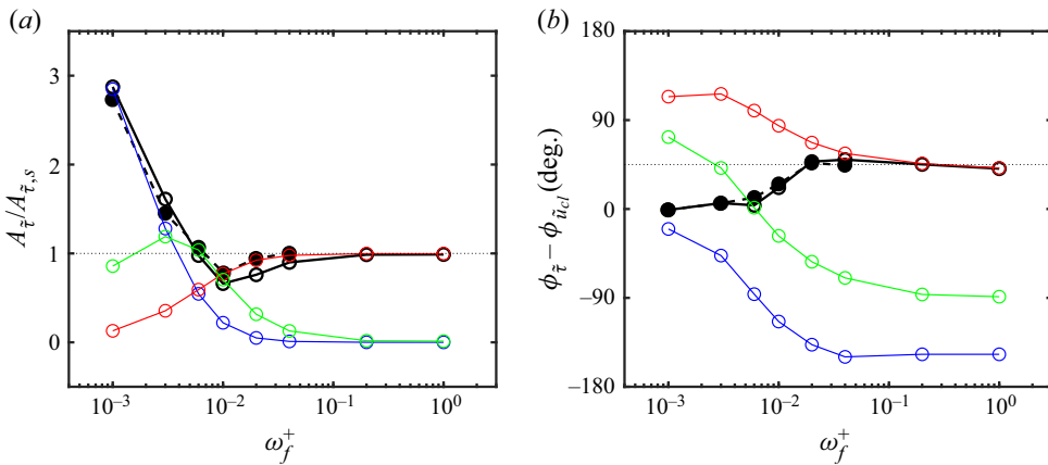
Figure 10. (a) The periodic wall-stress amplitude normalized by the Stokes solution. (b) The periodic wall-stress phase relative to the centreline velocity phase. Line types correspond to the DNS of Weng et al. (2016) (filled circles connected with thick dashed black lines) and LES using the MTS wall model (open circles connected with thick solid black lines), with LaRTE (open circles connected with thick solid blue lines), lamNEQ (open circles connected with thick solid red lines), and turbNEQ (open circles connected with thick solid green lines) components. The thin dotted horizontal black lines correspond to the Stokes solution.
