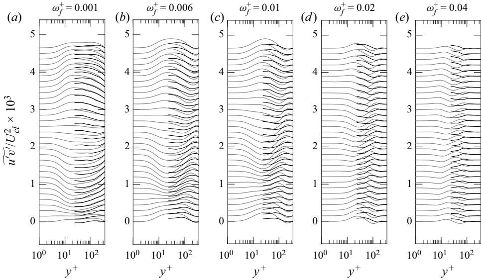
Figure 11. The time evolution of \widetilde{u'v'} at different phases of the wave cycle for different forcing frequencies: \omega_f^+ = 0.001, 0.006, 0.01, 0.02, 0.04 . The profiles are T_f/32 apart, and are offset by 1 \times 10^{-1} units in the vertical direction. Grey lines correspond to the DNS of Weng et al. (2016). Black lines correspond to LES using the MTS wall model. Animations of the different periodic Reynolds stress components can be viewed by clicking on the links corresponding to the following frequencies: \omega_f^+ = 0.001 , https://www.cambridge.org/S0022112023005852/JFM-Notebooks/files/Figure-11/rs_pul1_animation.html ; \omega_f^+ = 0.006 , https://www.cambridge.org/S0022112023005852/JFM-Notebooks/files/Figure-11/rs_pul3_animation.html ; \omega_f^+ = 0.01 , https://www.cambridge.org/S0022112023005852/JFM-Notebooks/files/Figure-11/rs_pul4_animation.html ; \omega_f^+ = 0.02 , https://www.cambridge.org/S0022112023005852/JFM-Notebooks/files/Figure-11/rs_pul5_animation.html ; \omega_f^+ = 0.04 , https://www.cambridge.org/S0022112023005852/JFM-Notebooks/files/Figure-11/rs_pul6_animation.html . The source code for generating these animations is located at https://www.cambridge.org/S0022112023005852/JFM-Notebooks/files/Figure-11/pulse_reynolds_stress_profiles.ipynb .
