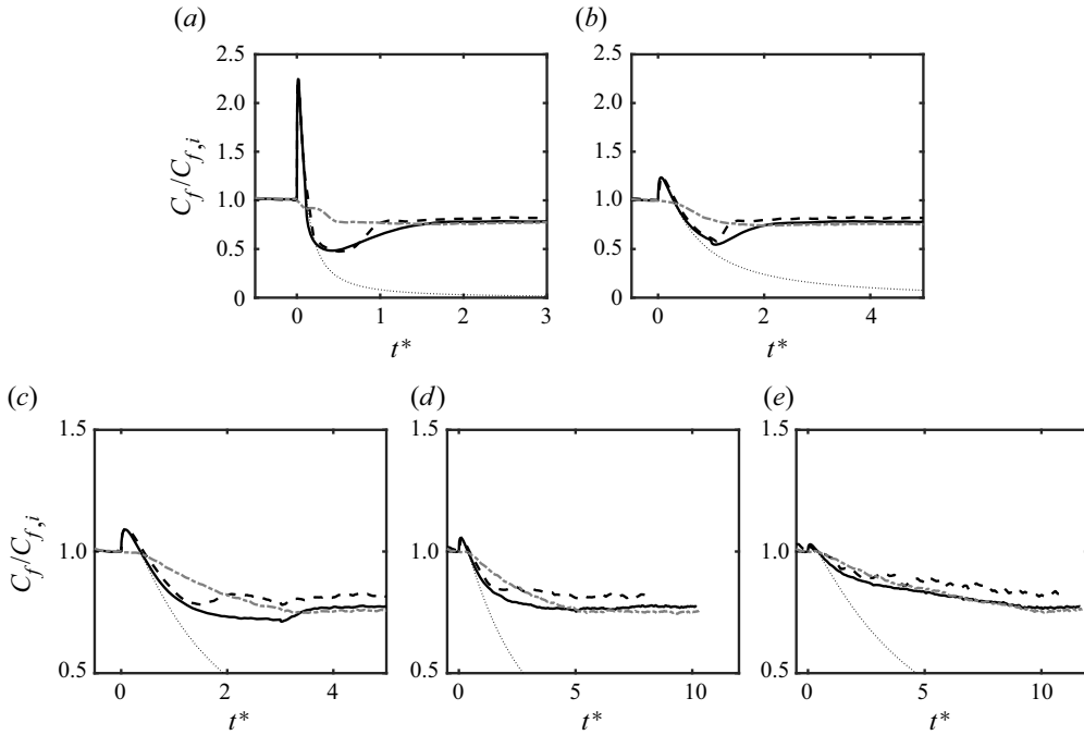
Figure 19. Time signals of the skin friction coefficient for different acceleration ramp rates. Ramp rates T^* = 0.1, 1.0, 3.0, 5.0, 10.0 correspond to plots (a–e), respectively. The curves compared are the DNS of Weng et al. (2016) (thick dashed black line), LES with the EQWM (thick dashed-dot grey line), and LES with the MTS wall model (thick solid black line). The thin black dotted line is the laminar solution given by (4.7).
