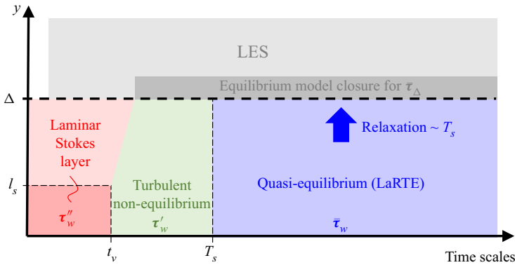
Figure 1. Multi-time-scale wall model length and time scales.
