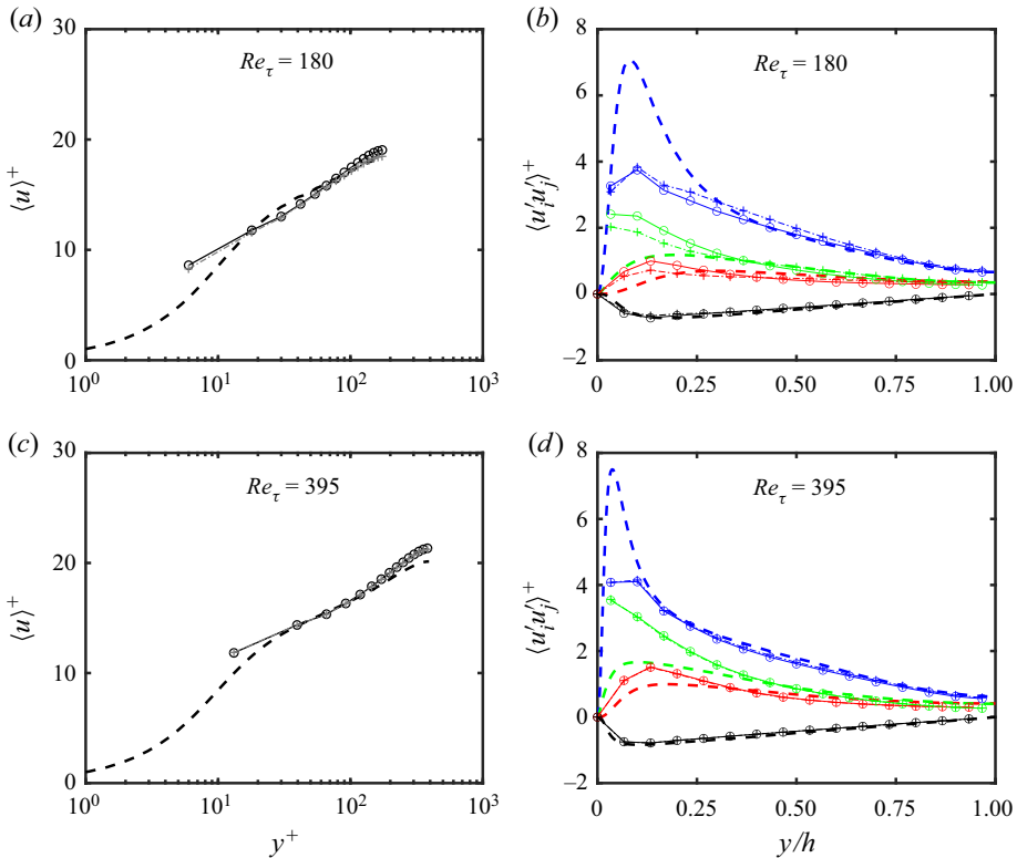
Figure 18. The mean velocity profiles and Reynolds stresses (a,b) before acceleration and (c,d) after acceleration, once the flow has achieved its new steady state. Dashed lines correspond to the DNS of Moser, Kim & Mansour (1999), circles with solid connecting lines correspond to LES with the MTS wall model, and plus signs with dashed-dot connecting lines correspond to LES with the EQWM. In (b,d), \langle u'u' \rangle , \langle v'v' \rangle , \langle w'w' \rangle and \langle u'v' \rangle are shown with blue, red, green and black lines, respectively.
