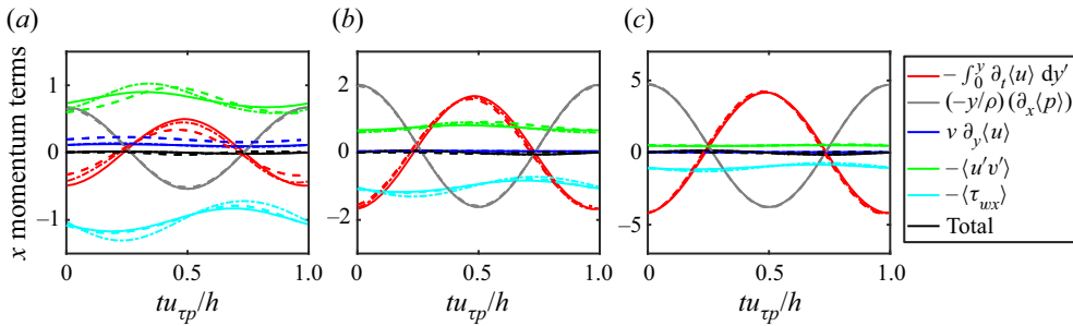
Figure 16. Time signals of budget terms for \omega_f^+ = 0.01 in the integrated, phase-averaged x momentum equation for different integration heights: (a) y/h = 0.067 , (b) y/h = 0.200 , and (c) y/h = 0.467 . Line types correspond to the DNS of Weng et al. (2016) (dashed lines), LES with the MTS wall model (solid lines), and LES with the EQWM (dashed-dot lines). Line colours correspond to different terms in the budget as indicated in the legend.
