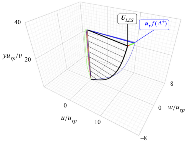
Figure 27. Assumed velocity profile below the wall-model grid point for the MTS wall-model approach. For an interactive animation of this sketch, see https://www.cambridge.org/S0022112023005852/JFM-Notebooks/files/Figure-27/steady_channel_flow_wm_velocity_profiles.html . (To play the animation, select ‘Controls’ and ‘Play loop’ on the K3D panel.) The source code that generated the animation can be found at https://www.cambridge.org/S0022112023005852/JFM-Notebooks/files/Figure-27/steady_channel_flow_wm_velocity_profiles.ipynb . Line colours for the total modelled velocity and its LaRTE, lamNEQ and turbNEQ components are black, blue, red and green, respectively. Thin coloured lines are the model’s streamwise and spanwise velocity profiles.
