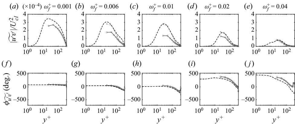
Figure 12. (a–e) Amplitude and (f–j) phase lead of \widetilde{u'v'} for five forcing frequencies, \omega_f^+ = 0.001, 0.006, 0.01, 0.02, 0.04 . The DNS of Weng et al. (2016), the LES with the MTS wall model, and the LES with the EQWM are shown with dashed lines, open circles with solid black connecting lines, and plus signs with grey dashed-dot connecting lines, respectively.
