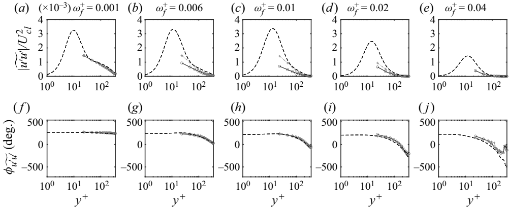
Figure 13. (a–e) Amplitude and (f–j) phase lead of \widetilde{u'u'} for five forcing frequencies \omega_f^+ = 0.001, 0.006, 0.01, 0.02, 0.04 . Line types are the same as in figure 12.
