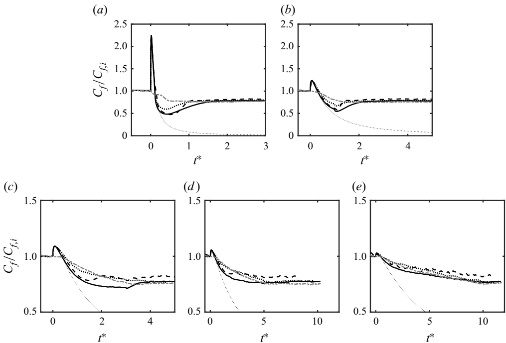
Figure 25. Time signals of the skin friction coefficient for different acceleration ramp rates. Ramp rates T^* = 0.1, 1.0, 3.0, 5.0, 10.0 correspond to plots (a–e), respectively. The curves compared are the DNS of Weng et al. (2016) (thick dashed black line), LES with the EQWM (thick dashed-dot grey line), LES with the EQMTS wall model (thick dotted black line), and LES with the MTS wall model (thick solid black line). The thin black dotted line is the laminar solution given by (4.7).
