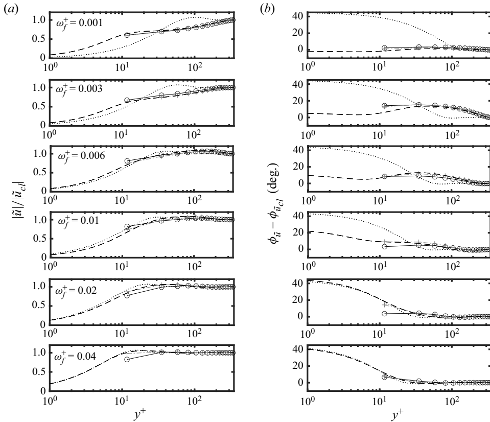
Figure 6. (a) Amplitude and (b) phase lead of the periodic velocity for six forcing frequencies, \omega_f^+ = 0.001, 0.003, 0.006, 0.01, 0.02, 0.04 . The DNS of Weng et al. (2016), the LES with the MTS wall model, the LES with the EQWM, and the Stokes solution are shown with dashed black lines, open circles connected with solid black lines, grey plus symbols connected with grey dashed-dot lines, and dotted black lines, respectively. Animations of the periodic velocity can be accessed at https://www.cambridge.org/S0022112023005852/JFM-Notebooks/files/Figure-6/u_animation.html , and the corresponding source code can be found at https://www.cambridge.org/S0022112023005852/JFM-Notebooks/files/Figure-6/pulse_velocity_profiles.ipynb . Note that the animations of the DNS velocity profiles are computed from the provided amplitudes and phases.
