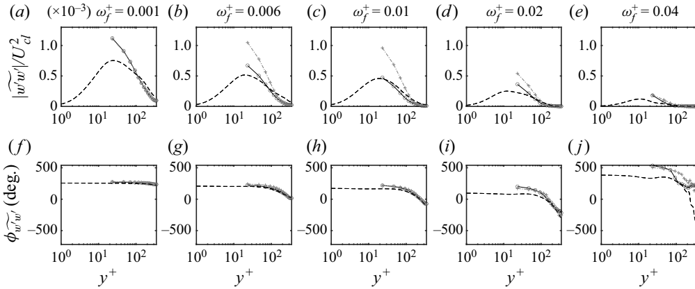
Figure 15. (a–e) Amplitude and (f–j) phase lead of w\tilde{w}' for five forcing frequencies, \omega_f^+ = 0.001, 0.006, 0.01, 0.02, 0.04 . Line types are the same as in figure 12.
