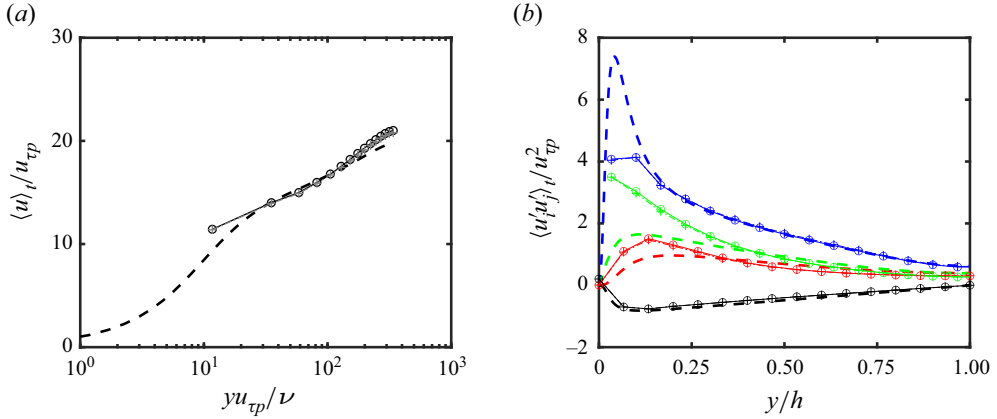
Figure 5. The time-averaged mean (a) velocity profiles and (b) Reynolds stresses. Dashed lines correspond to the DNS of Weng et al. (2016) for Re_{\tau} = 350 with pulsations; circles with solid connecting lines correspond to LES with the MTS wall model; and plus symbols with dashed-dot connecting lines correspond to LES with the EQWM. In (b), \langle u' u' \rangle_t , \langle v' v' \rangle_t , \langle w' w' \rangle_t and \langle u' v' \rangle_t are shown with blue, red, green and black lines, respectively. For the LES, only the high-frequency case ( \omega_f^+ = 0.04 ) is shown since the time-averaged velocity and Reynolds stress profiles are independent of the pulsation frequency.
