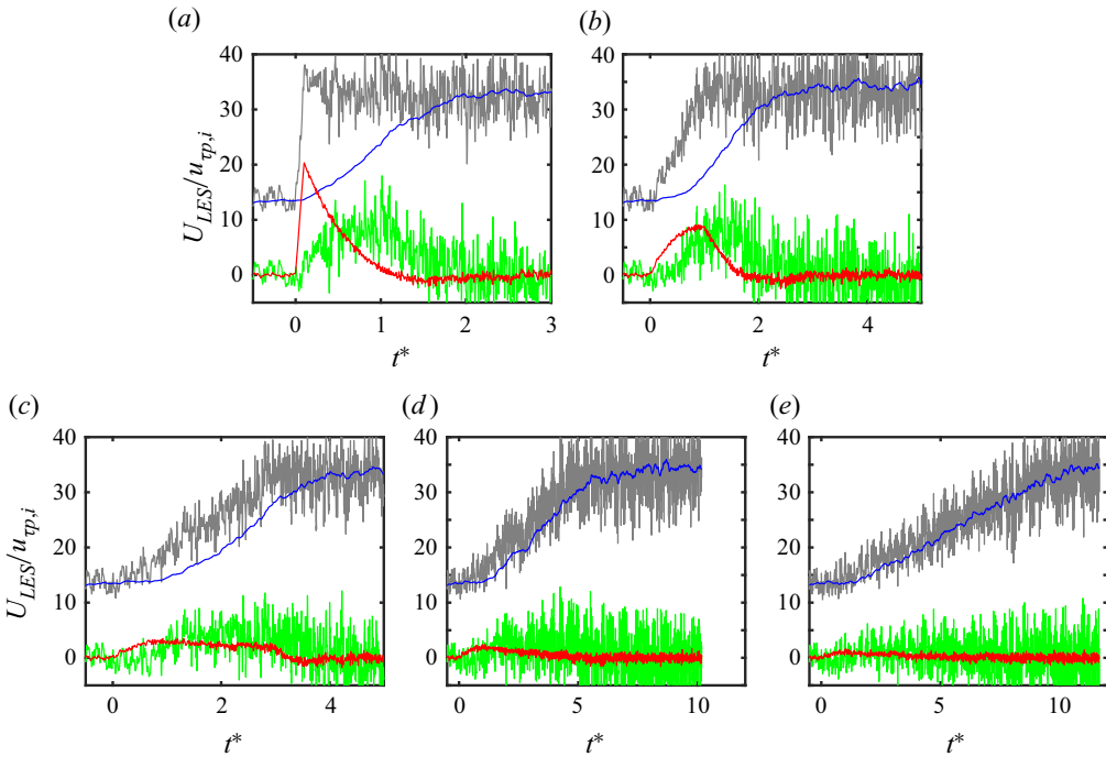
Figure 21. Time signals at a representative single point (x, y, z) = (L_x/2, \Delta, L_z/2) of the different modelling components of the LES velocity for several acceleration ramp rates. Ramp rates T^* = 0.1, 1.0, 3.0, 5.0, 10.0 correspond to plots (a–e), respectively. The different lines correspond to U_{LES} , u_{\tau f}(\Delta^+) , u'_{\Delta} and u''_{\Delta} , shown in grey, blue, green and red, respectively.
