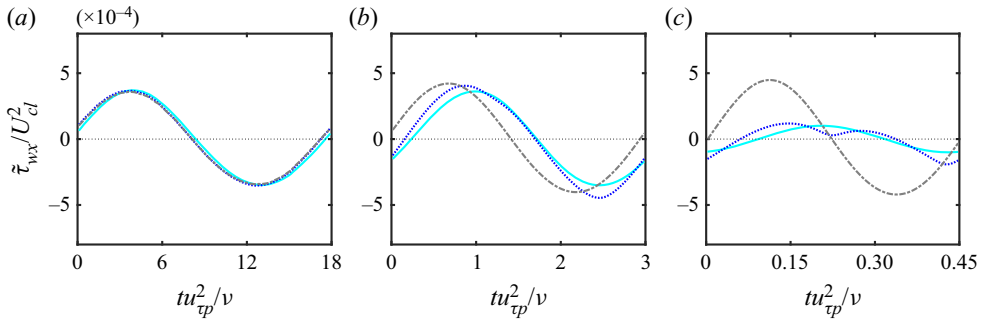
Figure 24. Single-period time evolution of the periodic streamwise wall stress \tilde{\tau}_{wx} for low, intermediate and high forcing frequencies, \omega_f^+ = 0.001, 0.006, 0.04 (plots (a–c), respectively). Curves shown include the corrected equilibrium component of the EQMTS wall model (dotted blue), the EQWM wall stress (dashed-dot grey), and the LaRTE+turbNEQ wall stresses (solid cyan). The phase within the cycle is based on the imposed forcing frequency.
