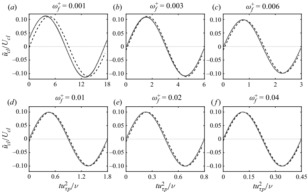
Figure 4. The time evolution of the periodic centreline velocity \tilde{u}_{cl} for several forcing frequencies, \omega_f^+ = 0.001, 0.003, 0.006, 0.01, 0.02, 0.04 (plots (a–f), respectively). Line types correspond to LES using the MTS wall model (thick solid black), LES using the EQWM (thick dashed-dot grey), and DNS from Weng et al. (2016) (thick dashed black). The phase within the cycle is based on the imposed pressure gradient forcing.
