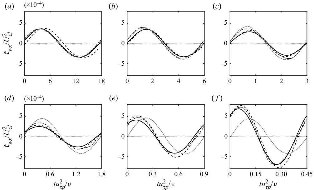
Figure 23. Single-period time evolution of the periodic streamwise wall stress \tilde{\tau}_{wx} for several forcing frequencies, \omega_f^+ = 0.001, 0.003, 0.006, 0.01, 0.02, 0.04 (plots (a–f), respectively). Line types correspond to LES using the MTS wall model (thick solid black), LES using the EQWM (thick dashed-dot grey), LES using the equilibrium MTS wall model (thick dotted black) and DNS from Weng et al. (2016) (thick dashed black). The phase within the cycle is based on the imposed forcing frequency.
