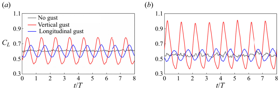
Figure 6. Time history of lift coefficients in different inflow conditions: (a) \alpha = 6^\circ ; (b) \alpha = 12^\circ .
