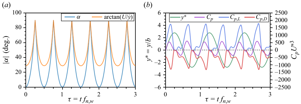
Figure 16. Time trace of (a) the absolute angle of attack and \arctan(U/\dot{y}) , and (b) the body displacement and instantaneous energy transfer between the cylinder and fluid for \{U^*, K_p^*, \phi_d\} = \{7.0, 1.36 \times 10^{-1}, 301^\circ\} .
