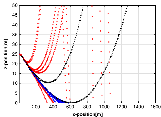
Figure 8 Case 2: Final flight profiles for a trial with no near-ground control switching, with wind
